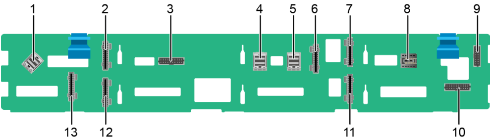
Figure 5-94 12 x 3.5" SAS/SATA/NVMe drive backplane
