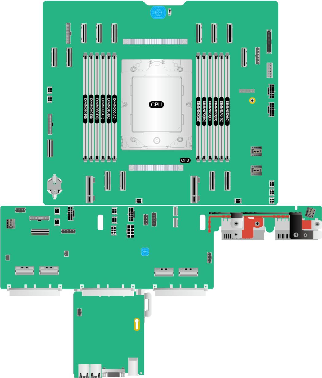
Figure 5-82 General-purpose server mainboard components
