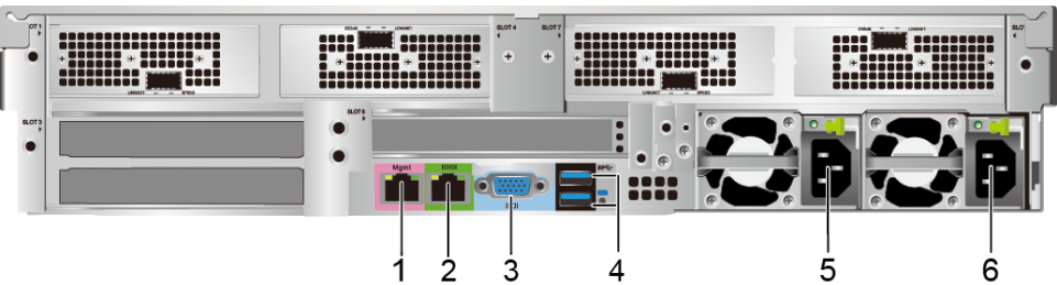
Figure 5-30 Ports on the rear panel
