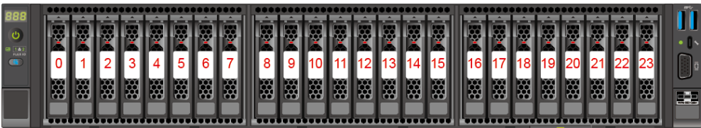
Figure 5-44 Drive number
