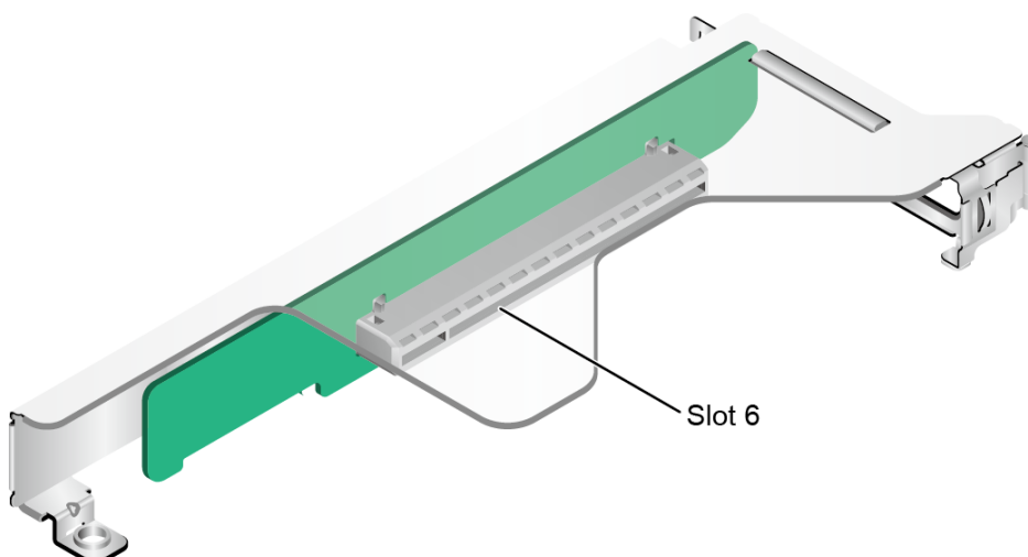
Figure 5-78 PCIe Riser card 5 (BC1M04PRUK)
