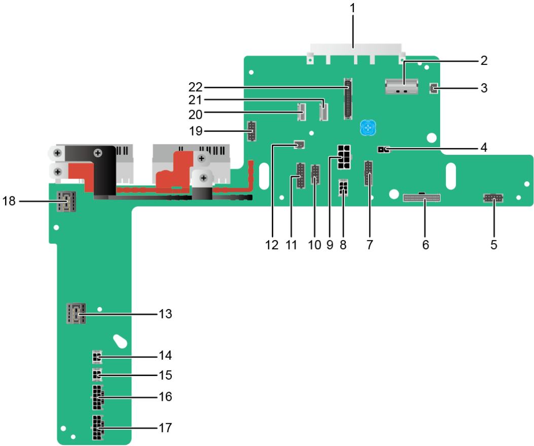
Figure 5-87 I/O expansion board of the 4-GPU server
