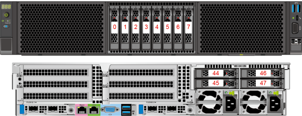
Figure 5-53 Drive number
