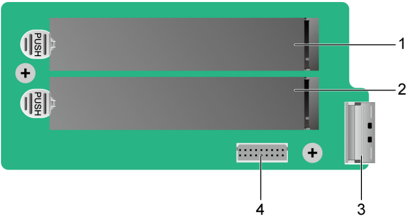
Figure 5-101 PCIe-SATA M.2 adapter card
