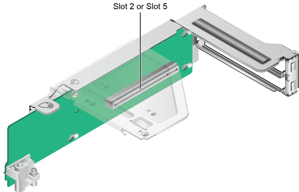
Figure 5-70 PCIe Riser card 3 (BC1M04PRUE)
