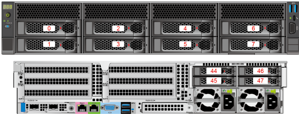
Figure 5-54 Drive number
