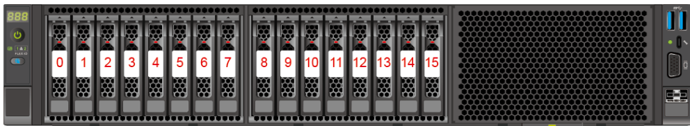
Figure 5-42 Drive number
