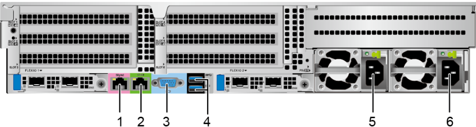
Figure 5-29 Ports on the rear panel
