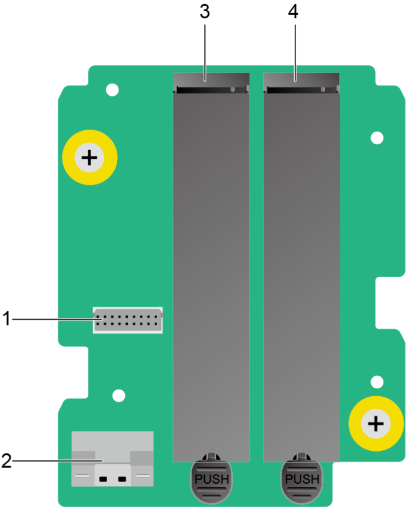
Figure 5-102 M.2 adapter card integrated in CPU
