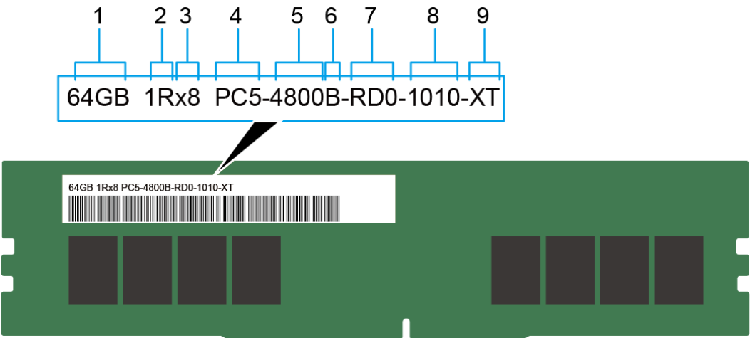
Figure 5-32 Memory identifier
