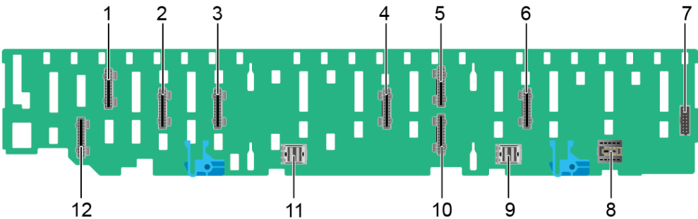
Figure 5-95 8 x SAS/SATA drives + 16 x NVMe drive pass-through backplane
