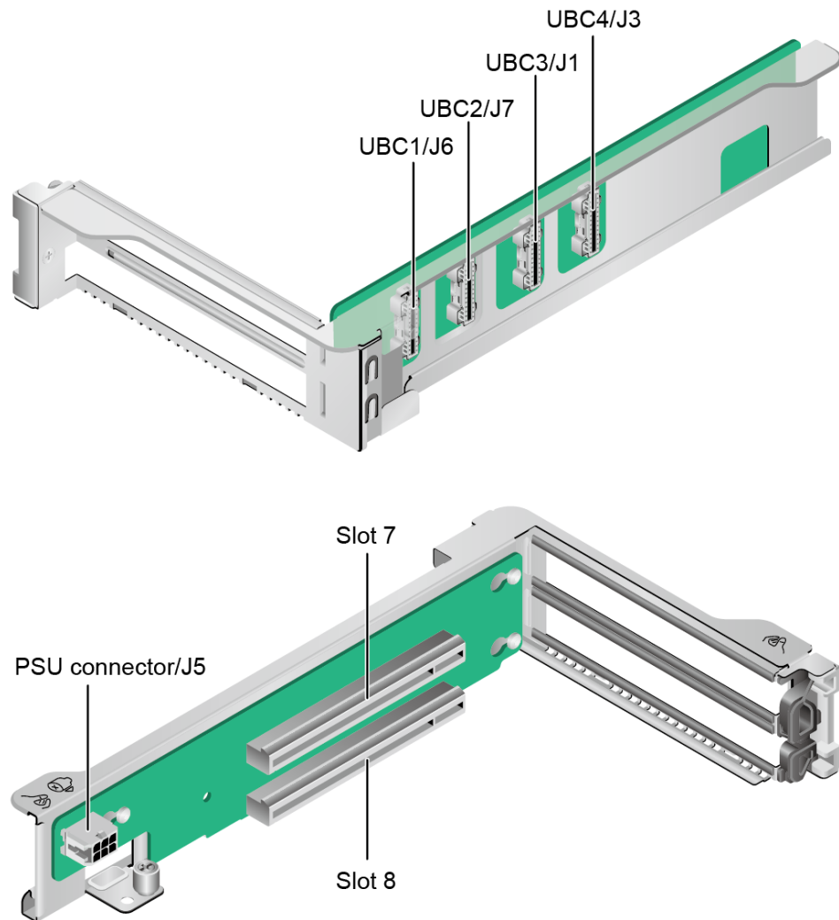
Figure 5-74 PCIe Riser card 1 (BC1M10PRUF)
