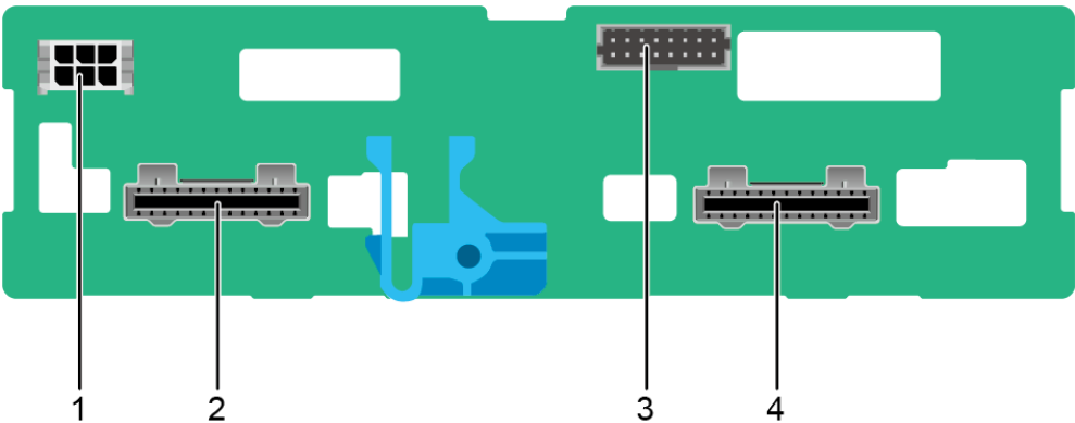
Figure 5-98 4 x NVMe drive backplane
