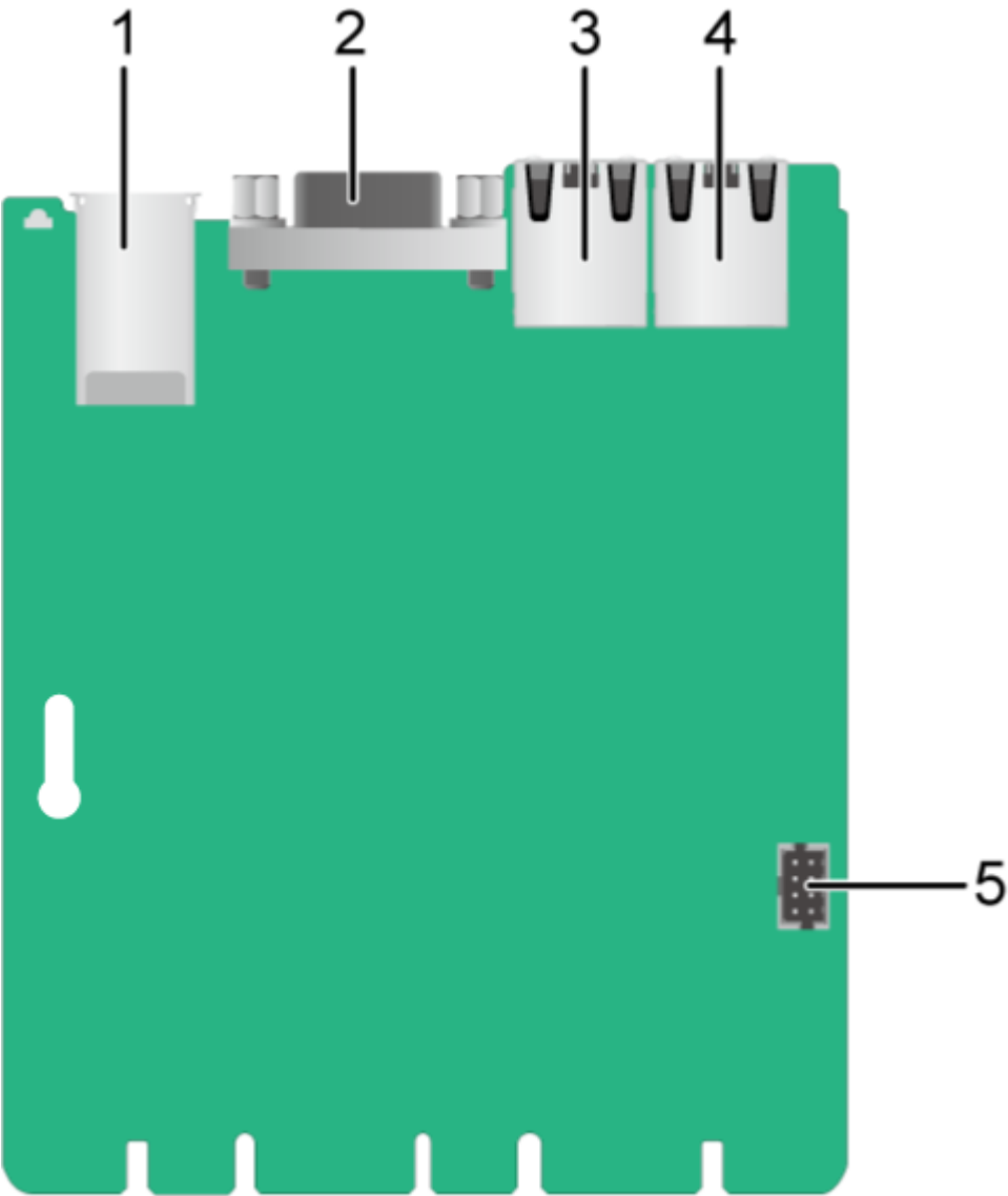
Figure 5-88 BMC card
