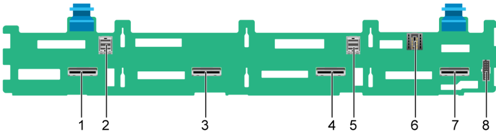
Figure 5-92 8 x 3.5" SAS/SATA/NVMe drive backplane
