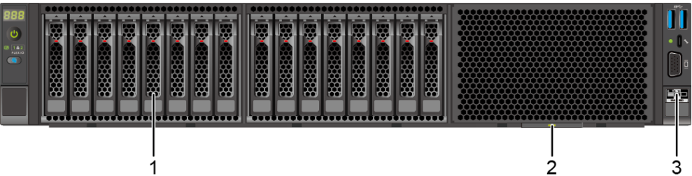
Figure 5-6 Front panel
