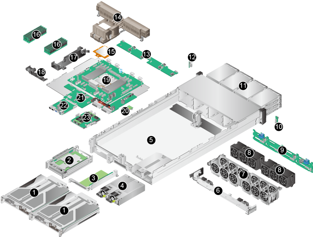
Figure 3-2 Physical structure of the 4-GPU server
