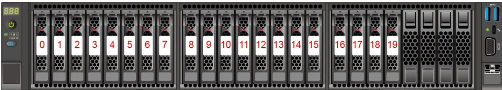
Figure 5-61 Drive number
