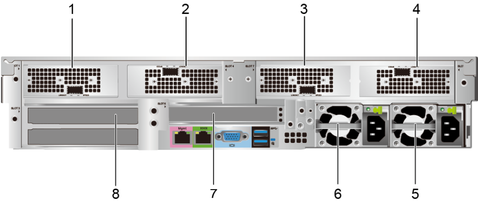
Figure 5-26 Rear panel
