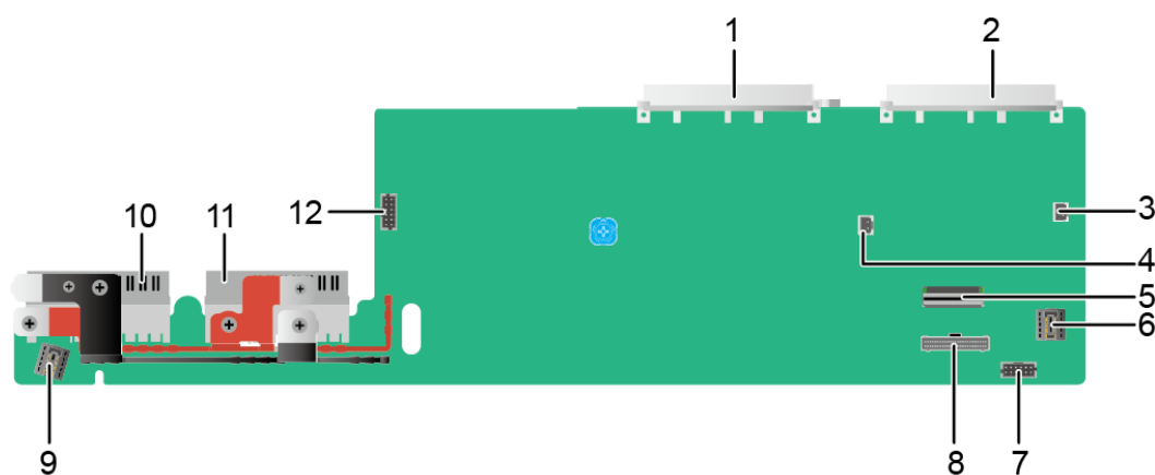
Figure 5-86 IO expansion board of general-purpose model (P/N code: 0302Y997)
