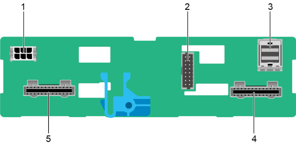
Figure 5-97 4 x 2.5" SAS/SATA/NVMe drive backplane
