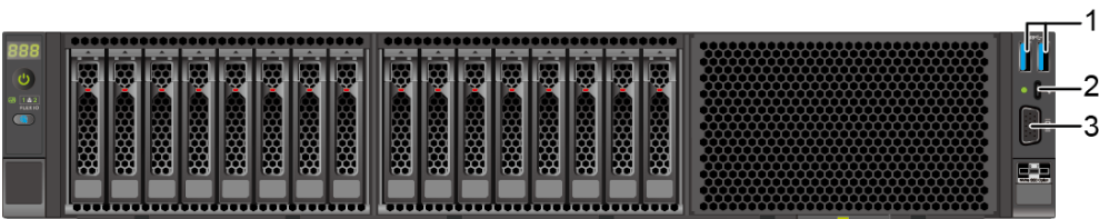
Figure 5-22 Ports on the front panel
