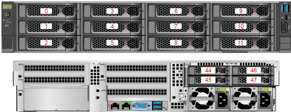
Figure 5-57 Drive number
