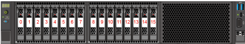
Figure 5-58 Drive number
