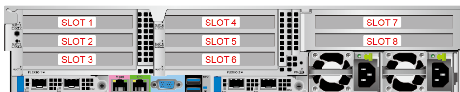
Figure 5-66 PCIe slots
