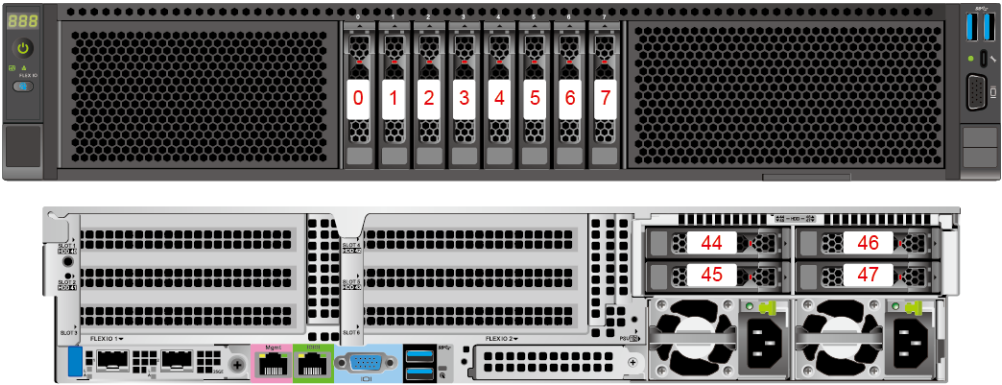
Figure 5-50 Drive number
