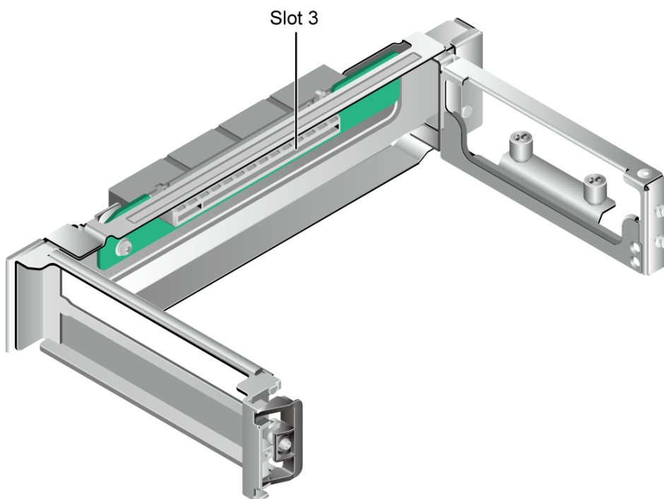
Figure 5-77 PCIe Riser module (BC1M01PRUWB)
