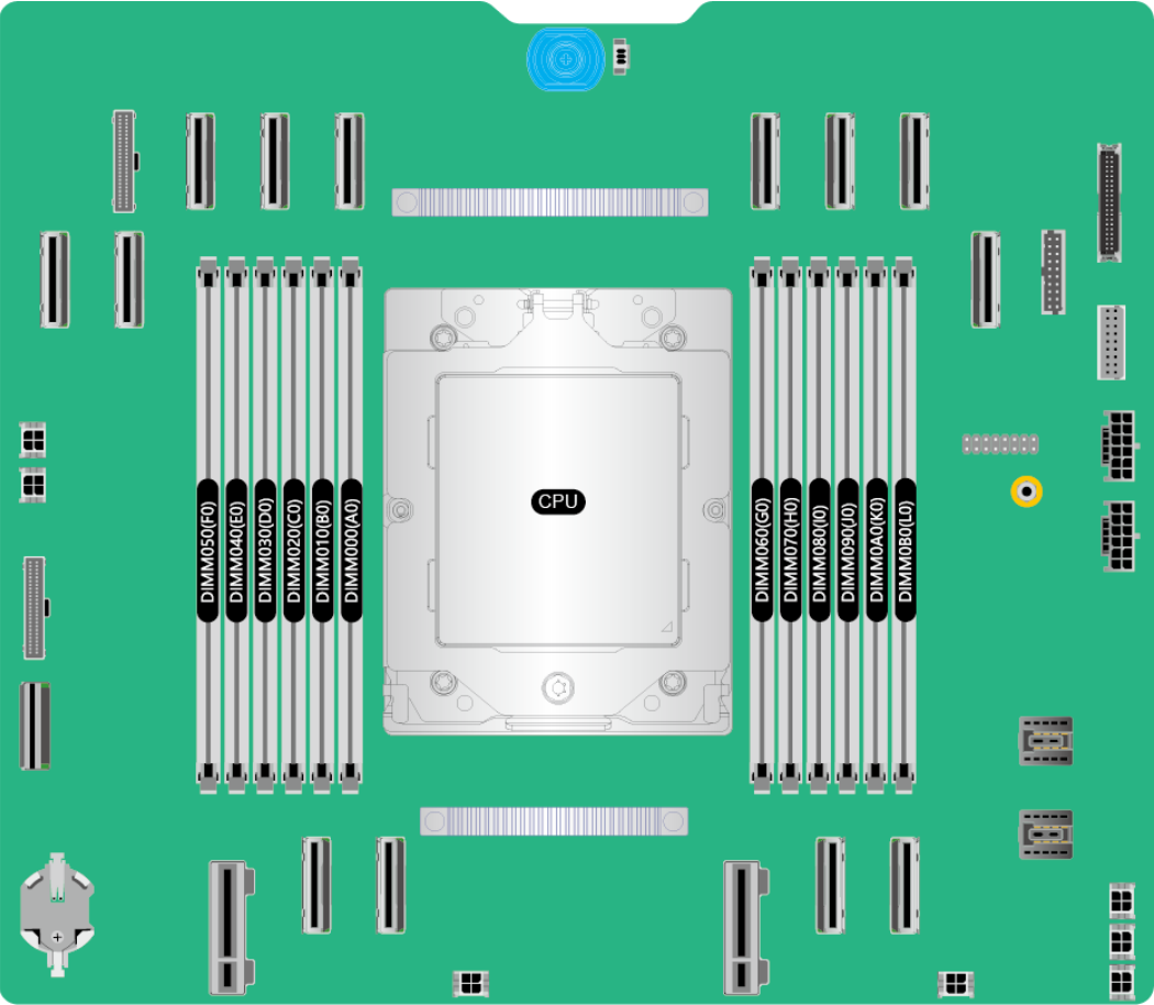
Figure 5-33 Positions of the memory modules
