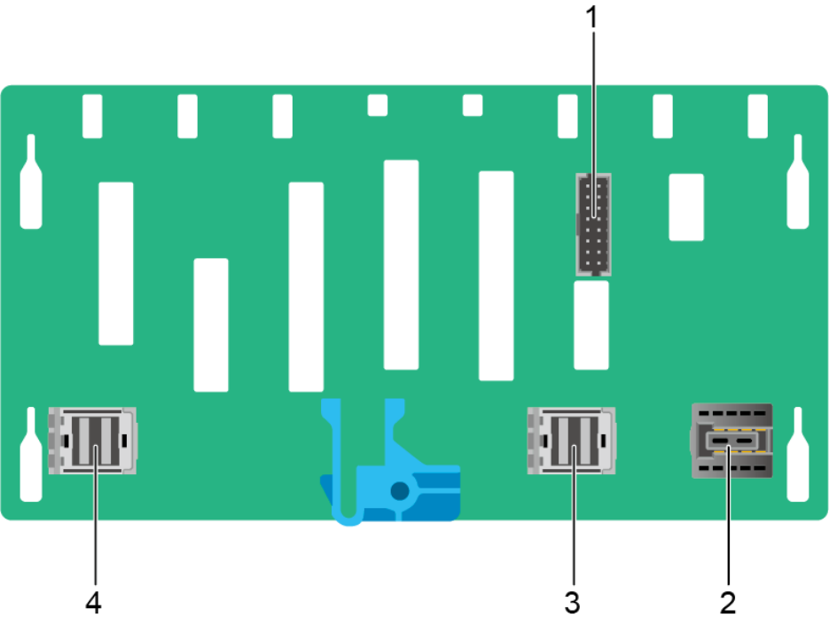
Figure 5-89 8 x 2.5" SAS/SATA drives pass-through backplane
