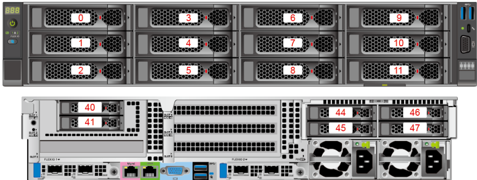
Figure 5-56 Drive number
