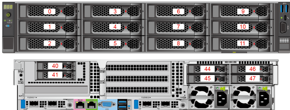
Figure 5-39 Drive number (I/O module 1 configured with 2.5" drives)
