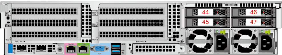
Figure 5-34 Drive number
