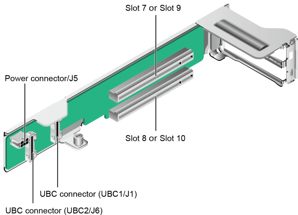
Figure 5-75 PCIe Riser module 2 (BC1M11PRUI)
