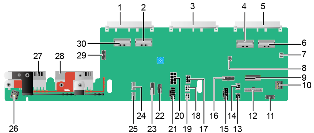
Figure 5-85 IO expansion board of general-purpose model (P/N code: 0302Y690)
