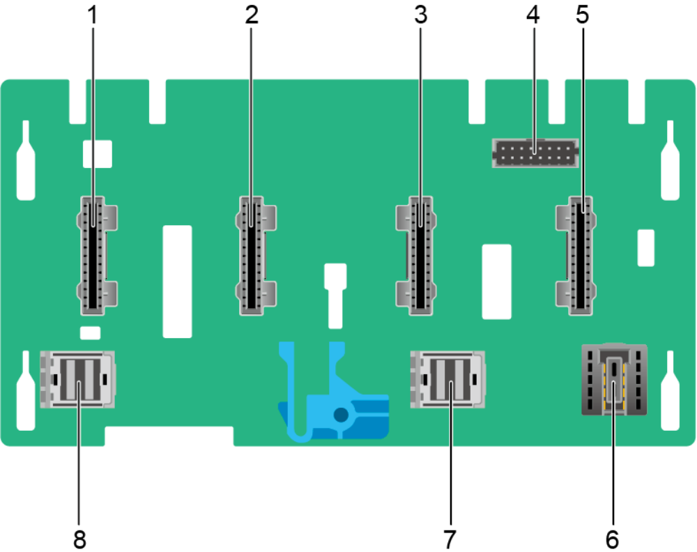
Figure 5-90 8 x 2.5" SAS/SATA/NVMe drive pass-through backplane
