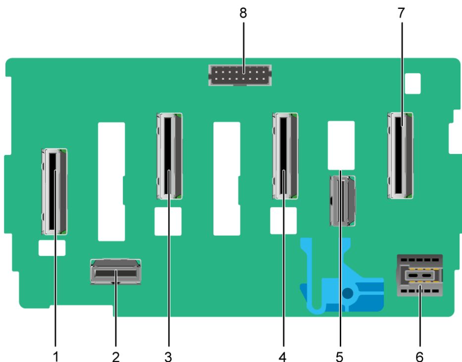
Figure 5-91 8 x 2.5" SAS/SATA/NVMe 3cage drive backplane
