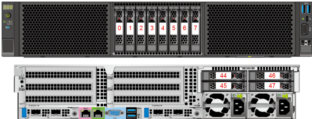
Figure 5-37 Drive number
