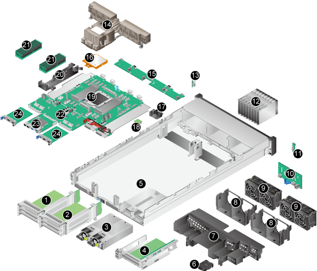
Figure 3-1 Physical structure of general-purpose server
