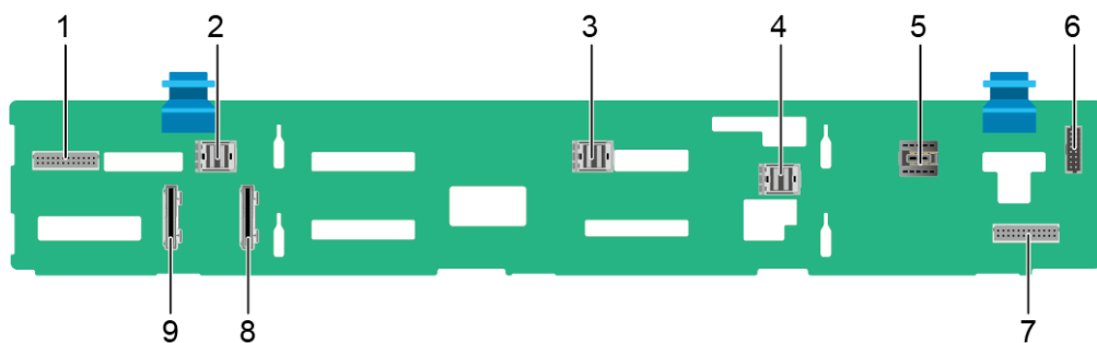
Figure 5-93 12 x 3.5" SAS/SATA/NVMe drives pass-through backplane
