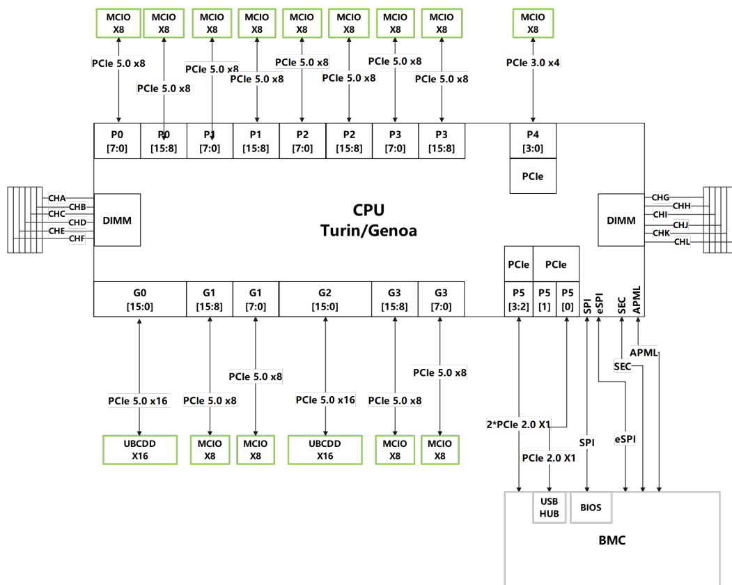
Figure 4-1 Logic structure
