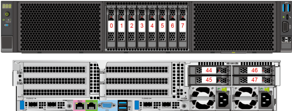
Figure 5-52 Drive number
