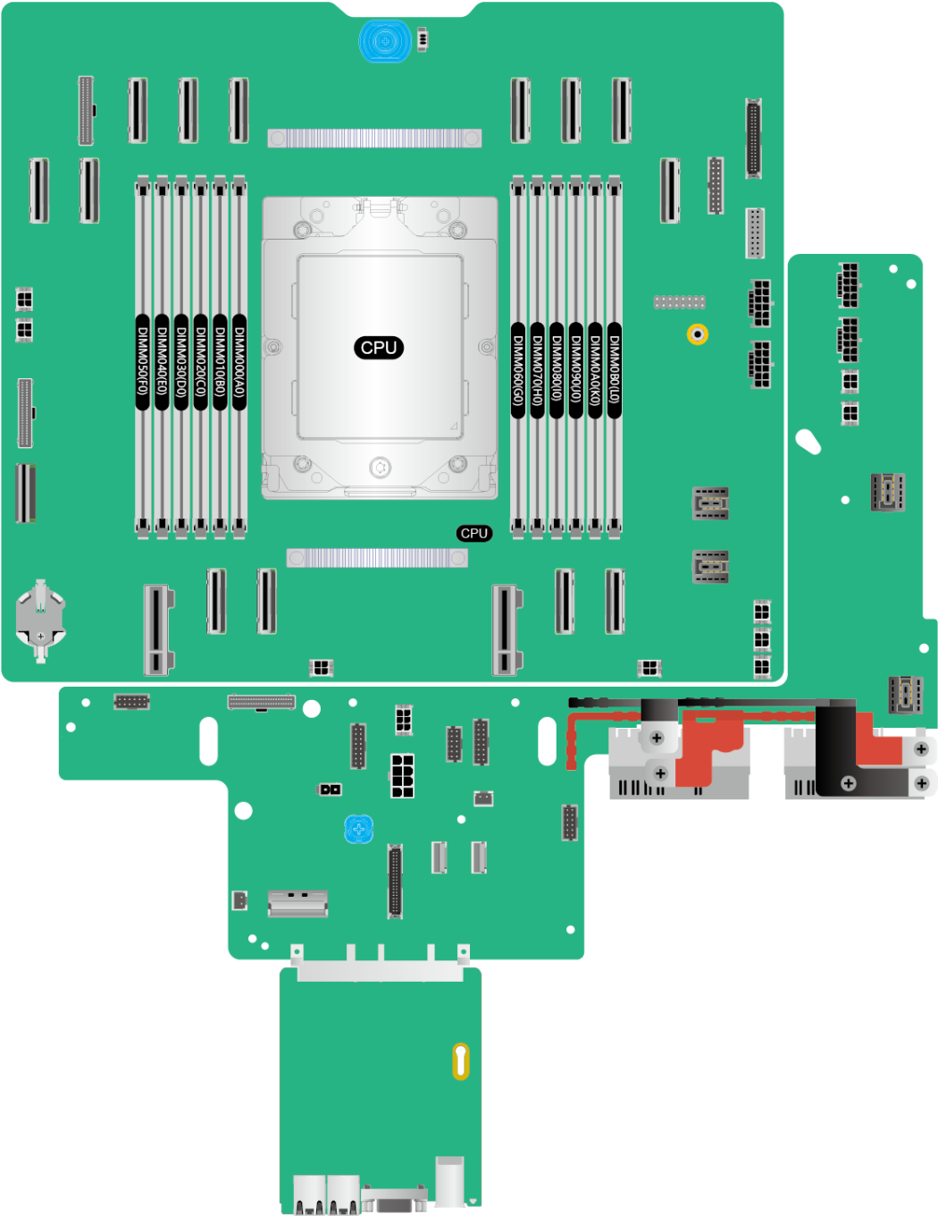
Figure 5-83 GPU server mainboard component
