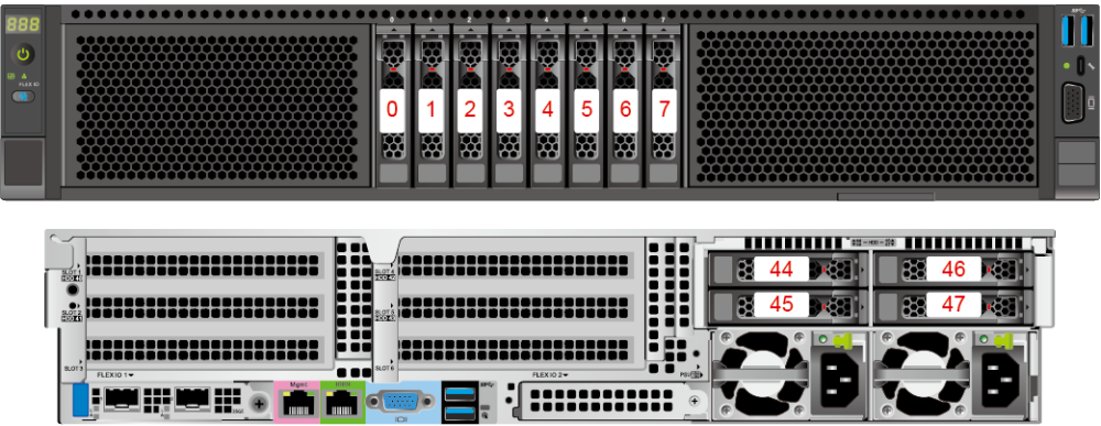
Figure 5-49 Drive number
