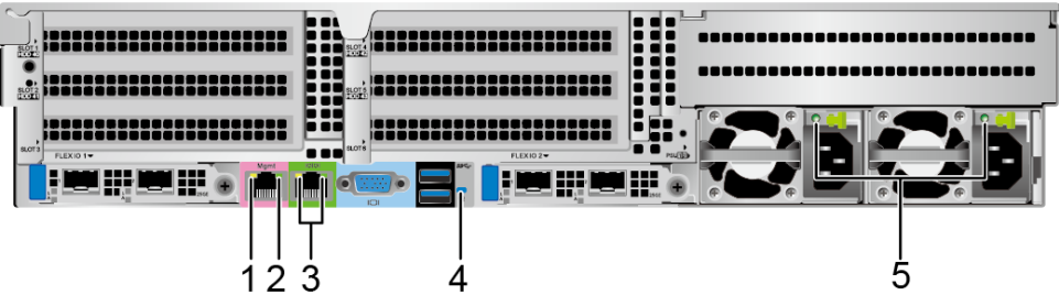
Figure 5-27 Indicators on the rear panel
