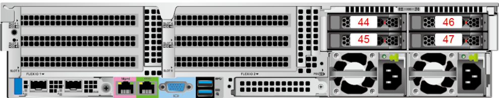
Figure 5-48 Drive number
