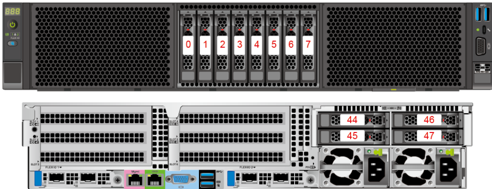
Figure 5-36 Drive number
