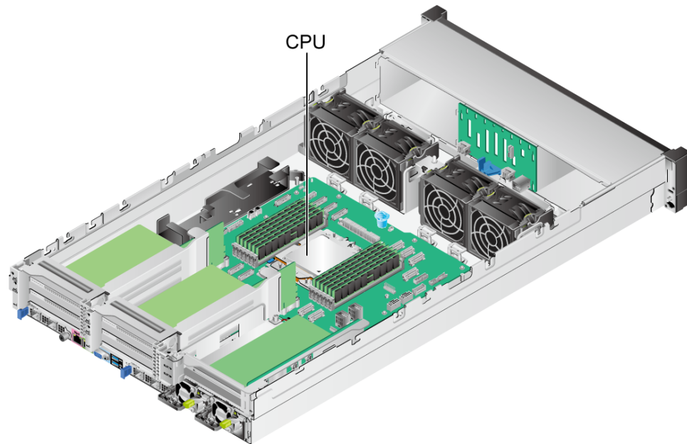
Figure 5-31 Positions of the processors
