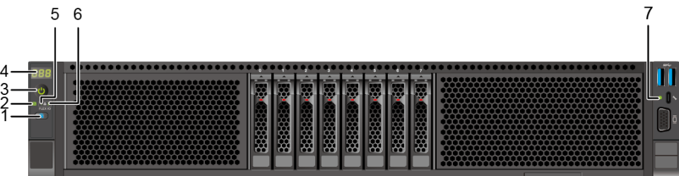
Figure 5-9 Indicators and buttons on the front panel
