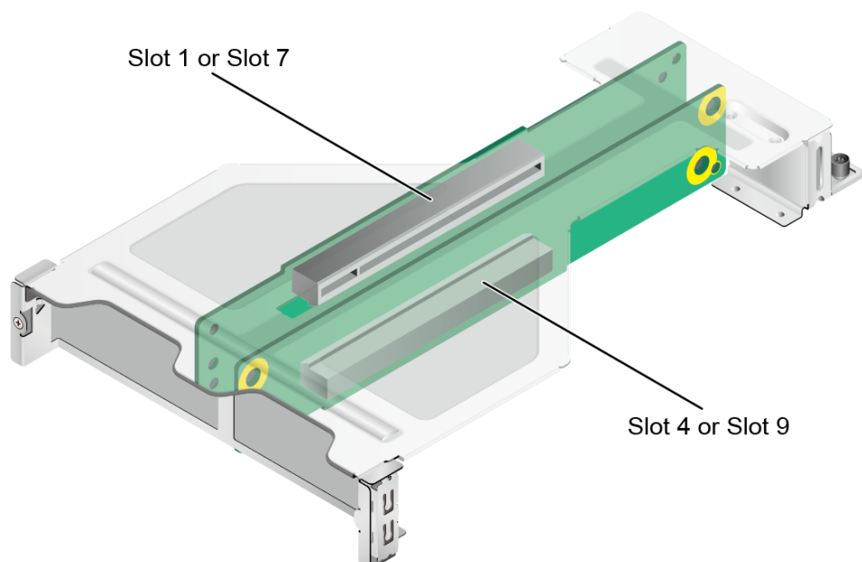
Figure 5-76 PCIe Riser card
