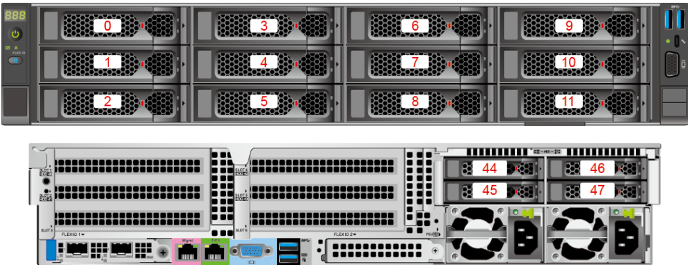
Figure 5-40 Drive number
