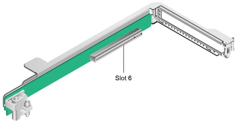
Figure 5-79 PCIe Riser card 6 (BC1M01PRUD)
