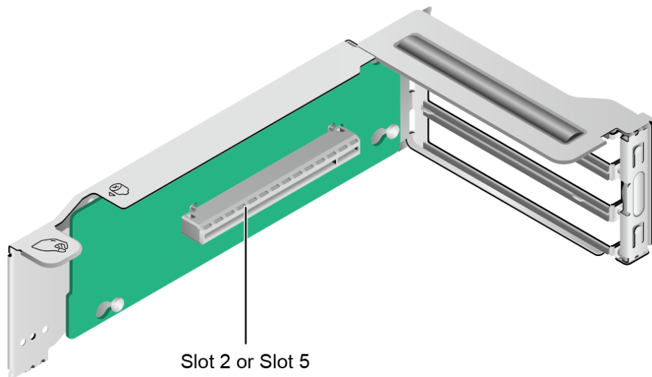
Figure 5-71 PCIe Riser card 4 (BC1M01PRUCC)
