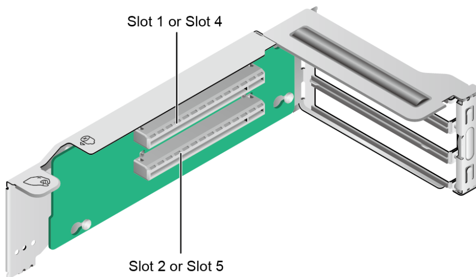
Figure 5-69 PCIe Riser card 2 (BC1M06PRUC)
