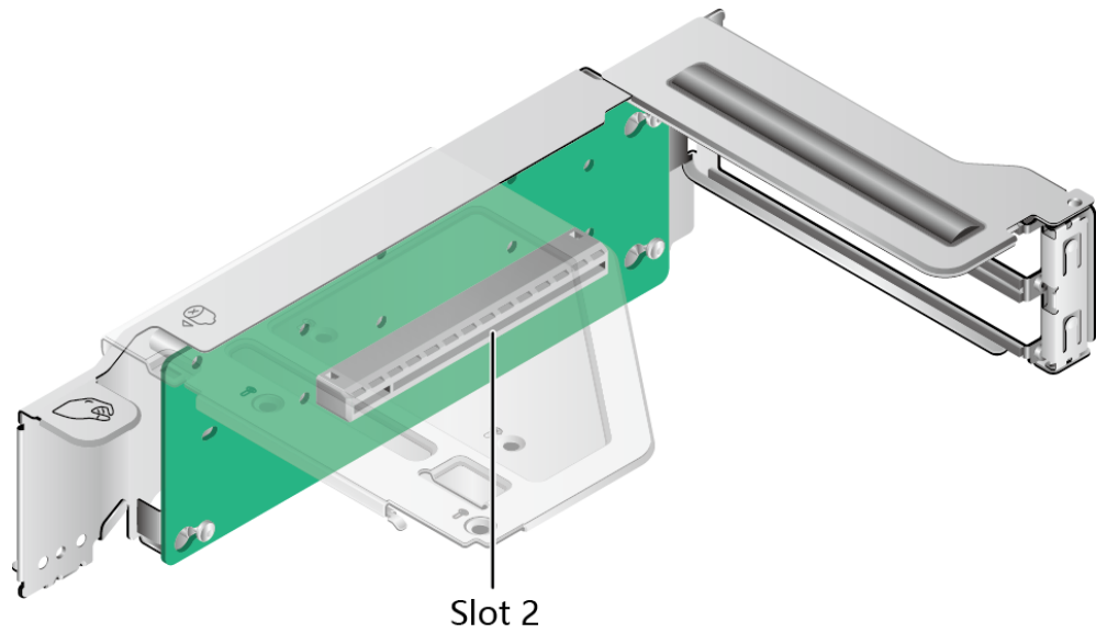
Figure 5-72 PCIe Riser card 5 (BC1M01PRUCB)
