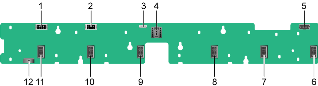
Figure 5-100 Fan board configured with 6056 fan modules
