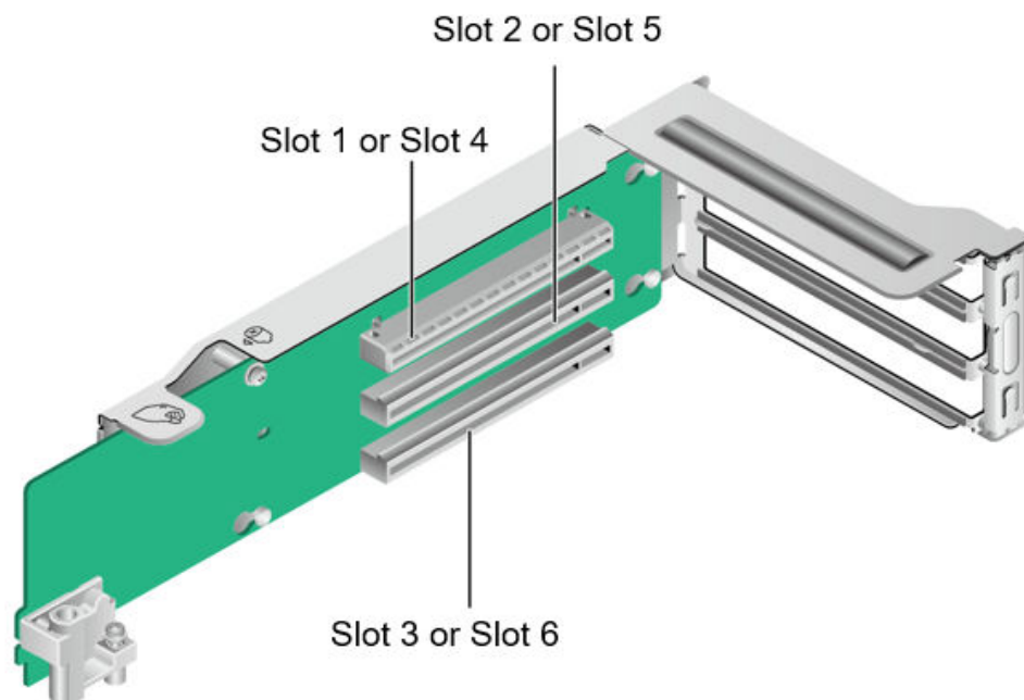
Figure 5-68 PCIe Riser card 1 (BC1M09PRUB)
