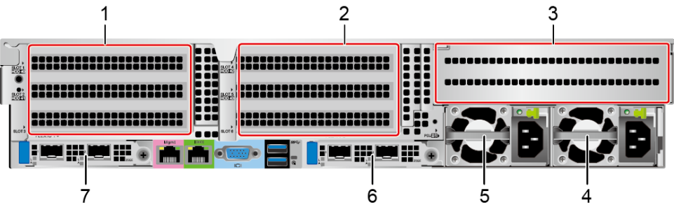
Figure 5-25 Rear panel
