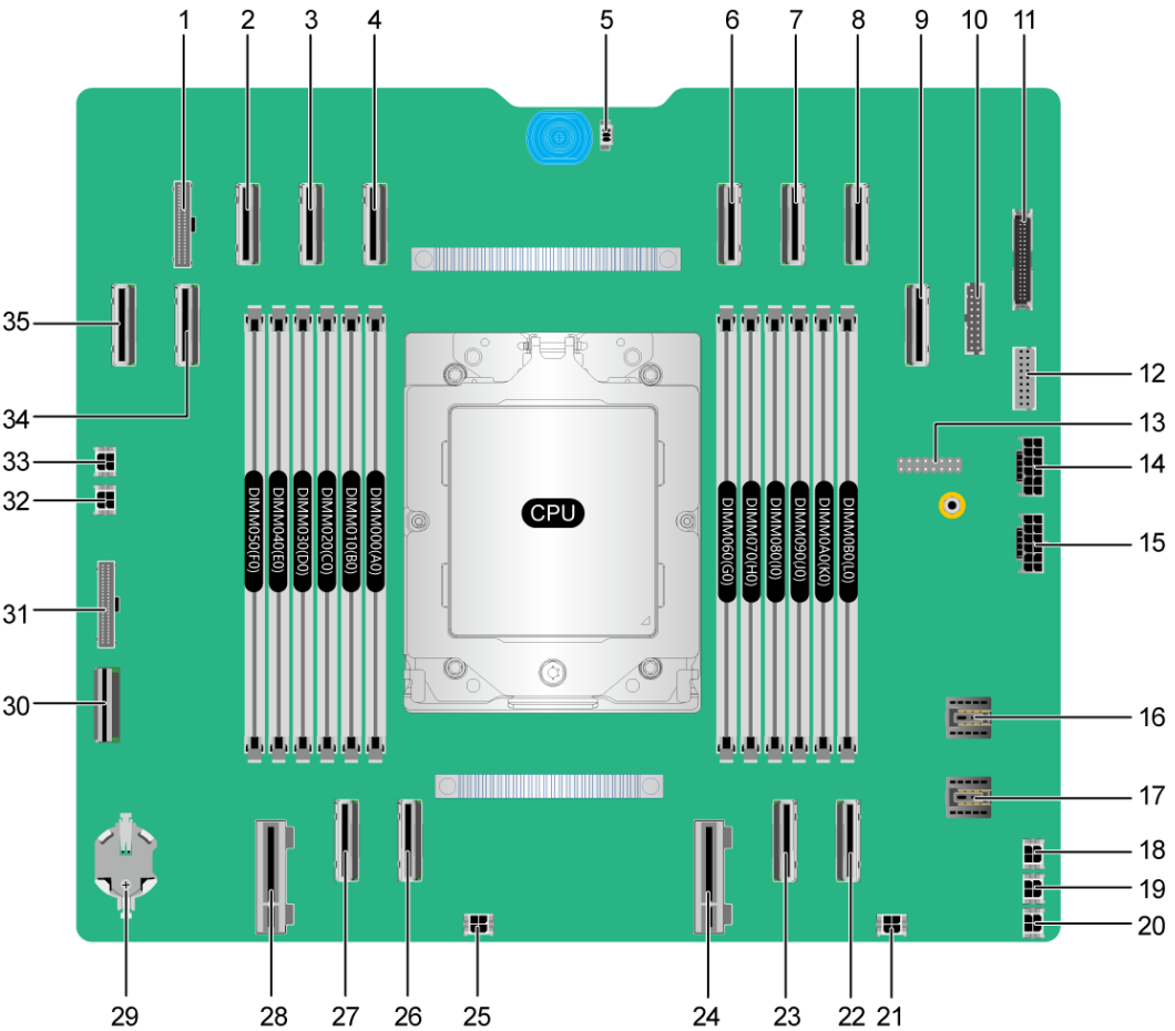
Figure 5-84 Mainboard
