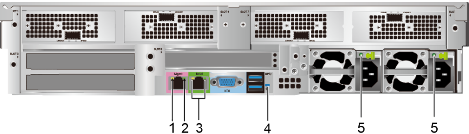
Figure 5-28 Indicators on the rear panel
