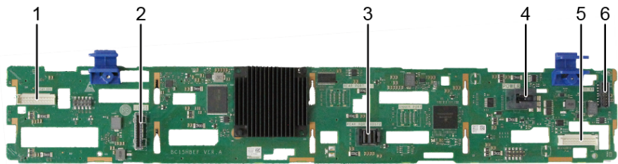
Figure 5-124 12 x 3.5" drive EXP backplane
