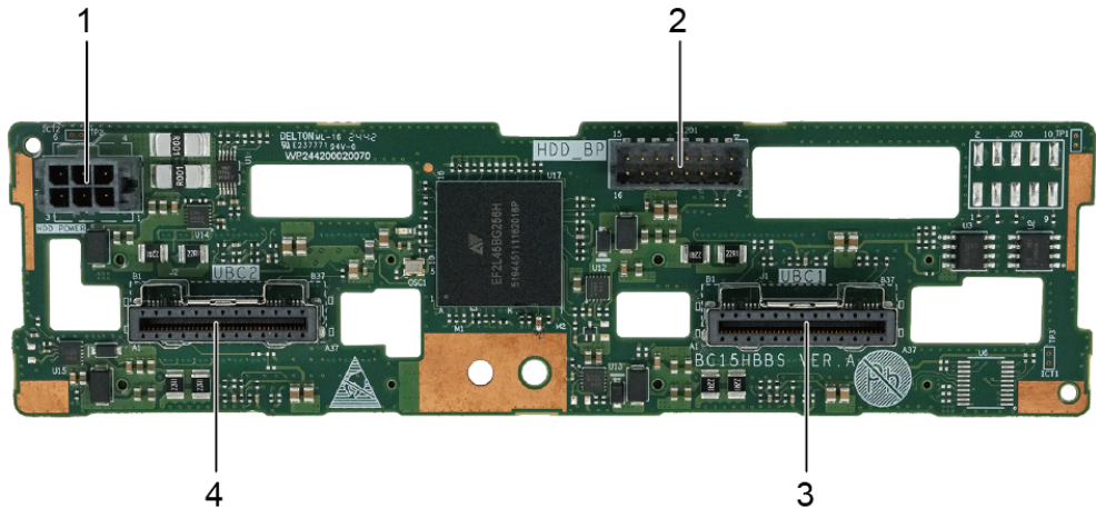
Figure 5-129 4 x 2.5" drive backplane 1
