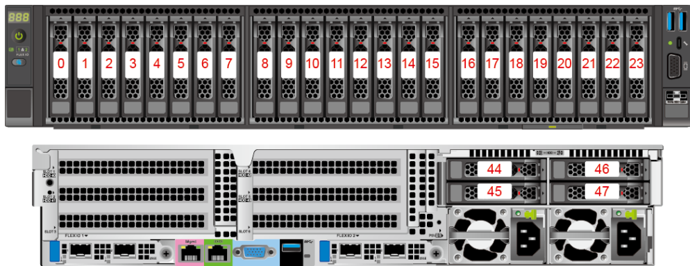
Figure 5-79 Drive number
