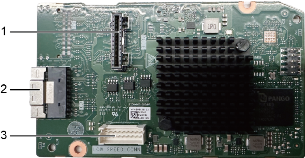
Figure 5-139 SATA Pass-through Card-8i
