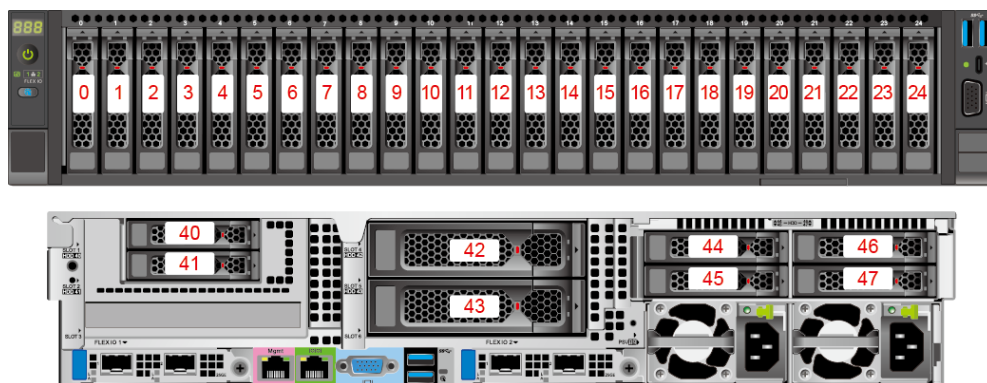
Figure 5-57 Drive numbers 2
