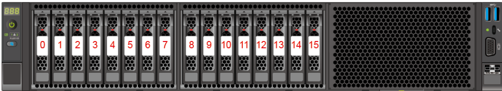
Figure 5-53 Drive numbers
