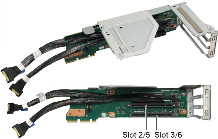
Figure 5-107 PCIe riser card 1 (BC16M02PRUL - supports cable card)
