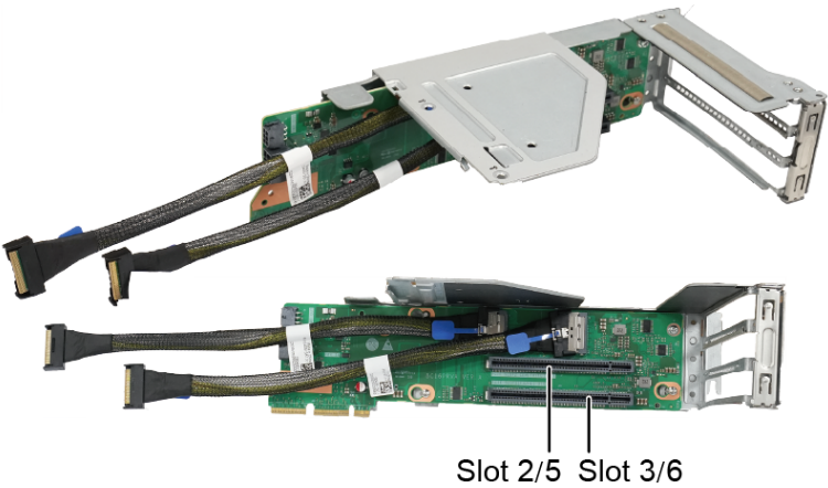
Figure 5-111 PCIe riser card 5 (BC16M01PRVA)
