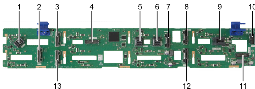
Figure 5-123 12 x 3.5" drive SAS/SATA/NVMe drive backplane
