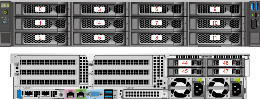
Figure 5-48 Drive numbers 3
