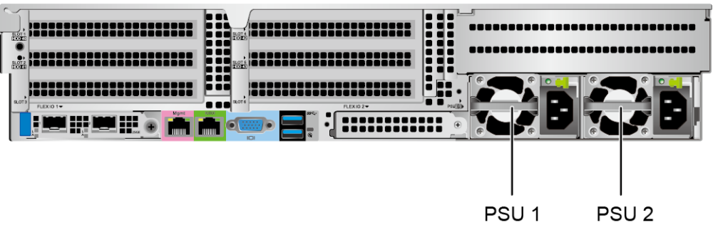
Figure 5-114 Position of the PSU
