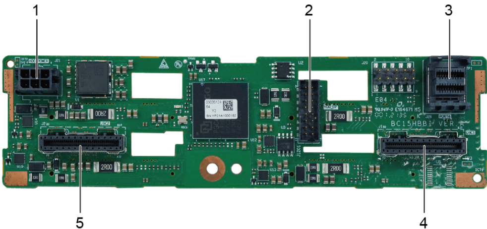
Figure 5-130 4 x 2.5" drive backplane 2
