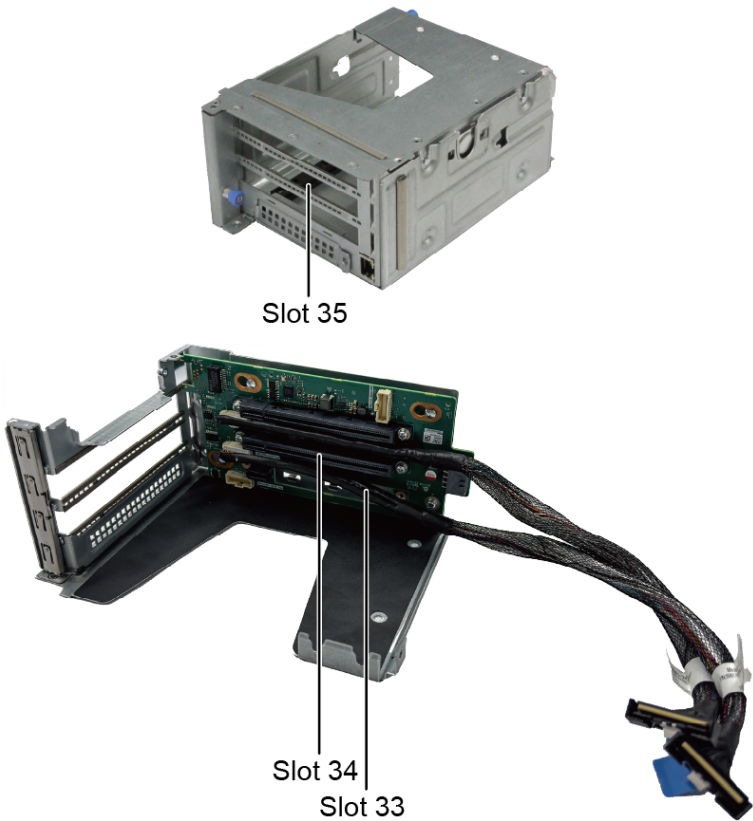
Figure 5-94 PCIe riser card 2
