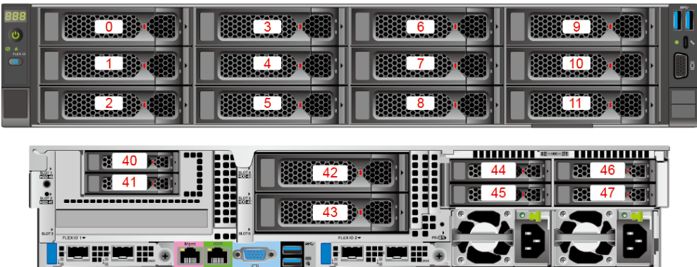
Figure 5-68 Drive numbers 2
