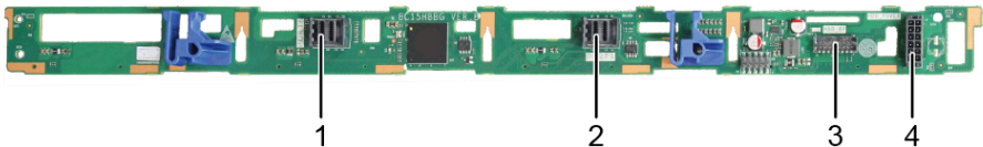
Figure 5-133 4 x 3.5" drive pass-through backplane
