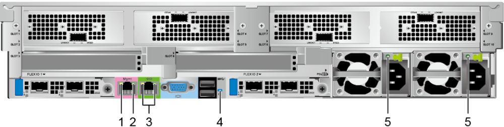
Figure 5-40 Indicators on the rear panel
