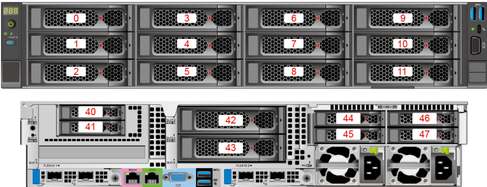
Figure 5-72 Drive numbers 2
