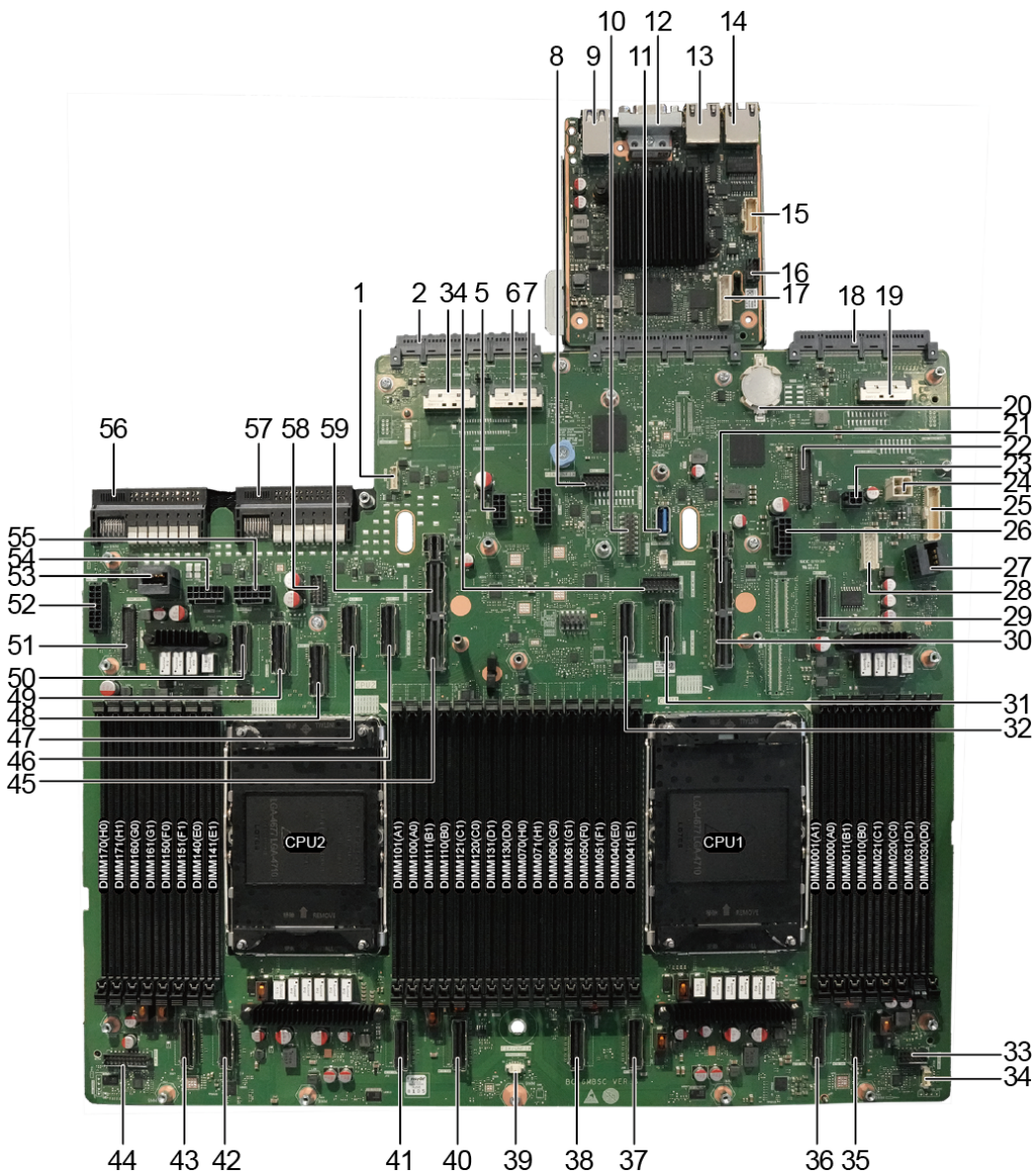
Figure 5-116 Mainboard
