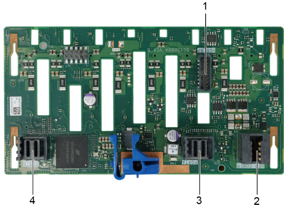
Figure 5-119 8 x 2.5" SAS/SATA common drive backplane
