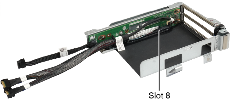
Figure 5-105 PCIe Riser card 2 of I/O module 3 (BC16M01PRUEA)
