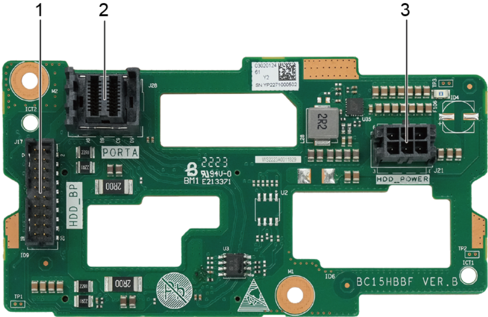
Figure 5-128 2 x 3.5" drive backplane
