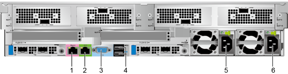
Figure 5-42 Ports on the rear panel
