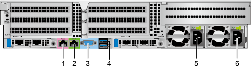
Figure 5-41 Ports on the rear panel
