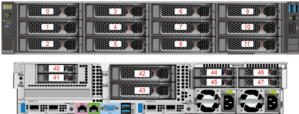
Figure 5-50 Drive numbers 2
