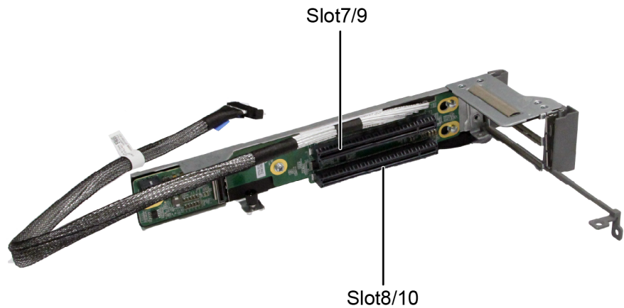
Figure 5-106 PCIe Riser card 3 of IO module 3 (BC16M01QHLHH)
