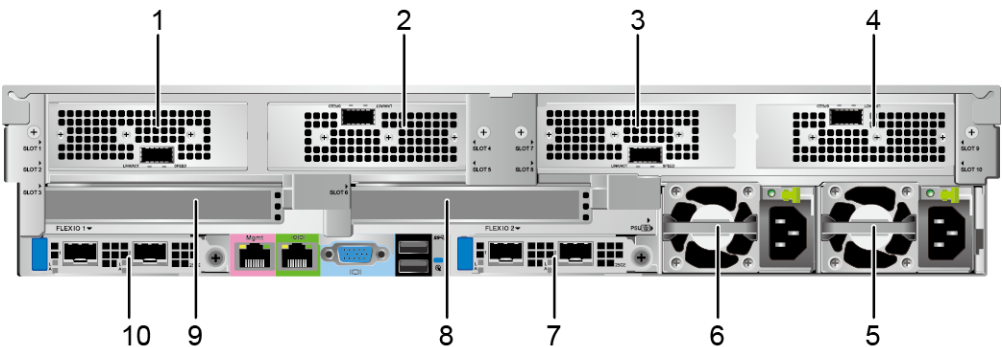
Figure 5-38 Rear panel
