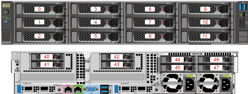
Figure 5-49 Drive numbers 1
