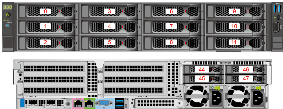
Figure 5-69 Drive numbers 3
