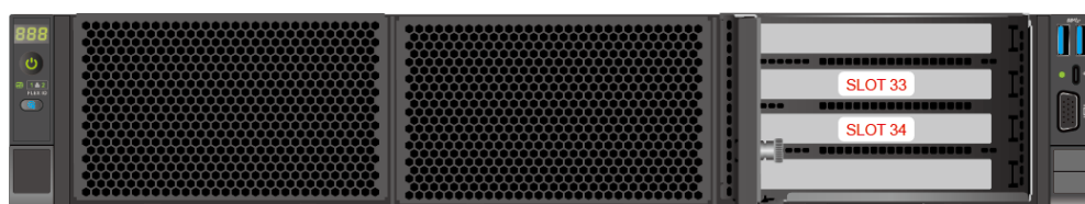
Figure 5-89 PCIe slots
