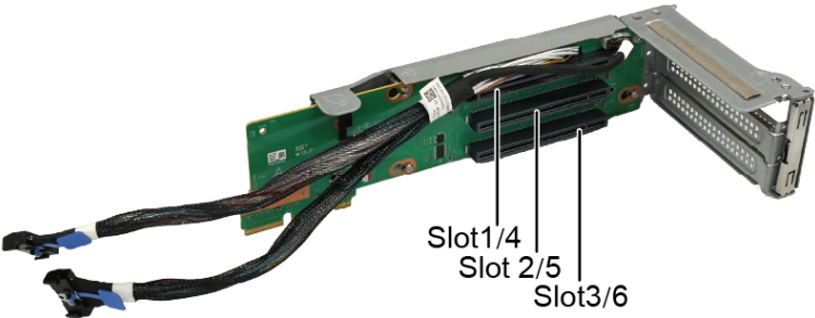
Figure 5-96 PCIe Riser card 1 (BC16M01PRUK)
