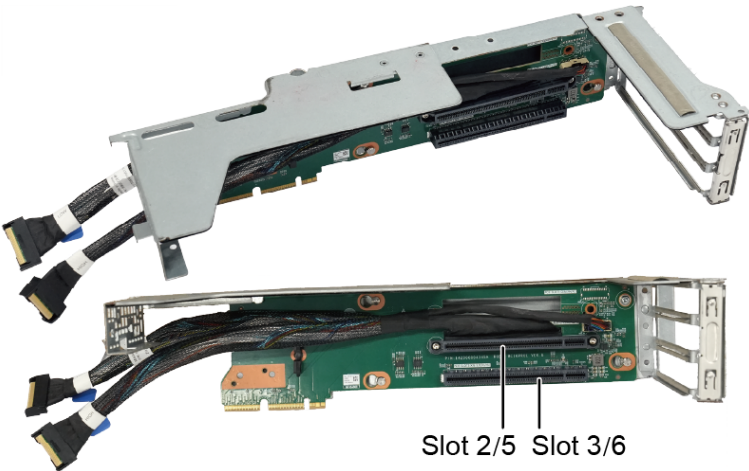
Figure 5-108 PCIe riser card 1 (BC16M03PRUL-supporting the full-length and dual-width GPU)
