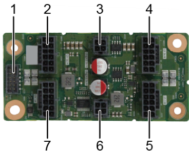
Figure 5-136 Power adapter board
