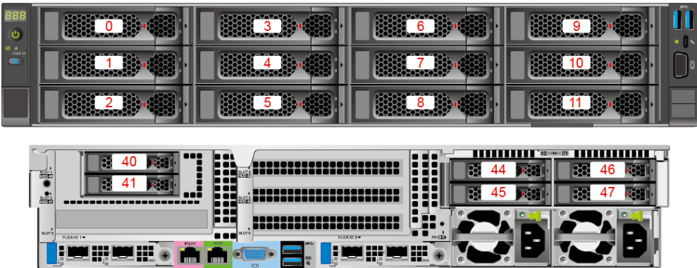
Figure 5-70 Drive numbers
