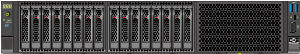
Figure 5-19 16 x 2.5" drive configuration 1
