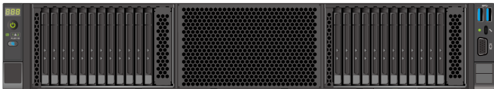
Figure 5-34 24 x E3.S 1 T pass-through configuration
