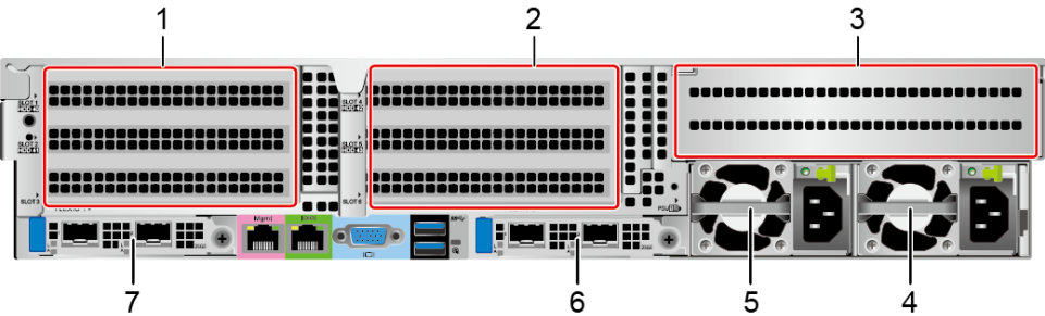
Figure 5-37 Rear panel
