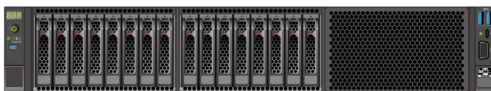
Figure 5-31 16 x 2.5" drive configuration 1
