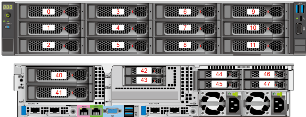
Figure 5-51 Drive numbers 3
