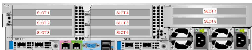
Figure 5-90 PCIe slots
