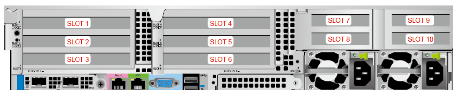
Figure 5-91 PCIe slots
