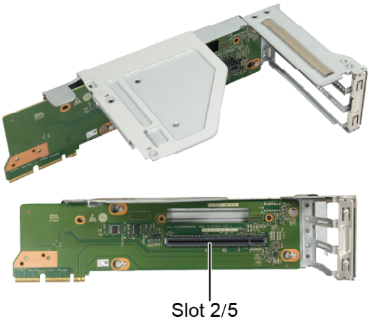
Figure 5-101 PCIe Riser card 6 for IO module 1/IO module 2 (BC16M01PRUIA)
