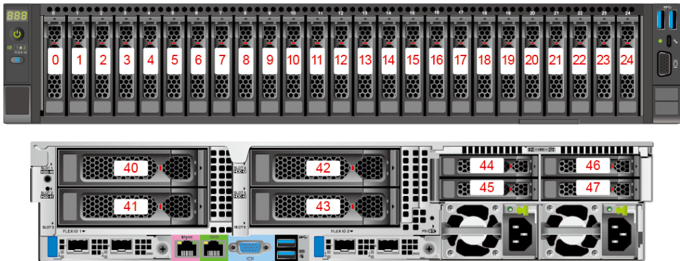
Figure 5-58 Drive numbers 3
