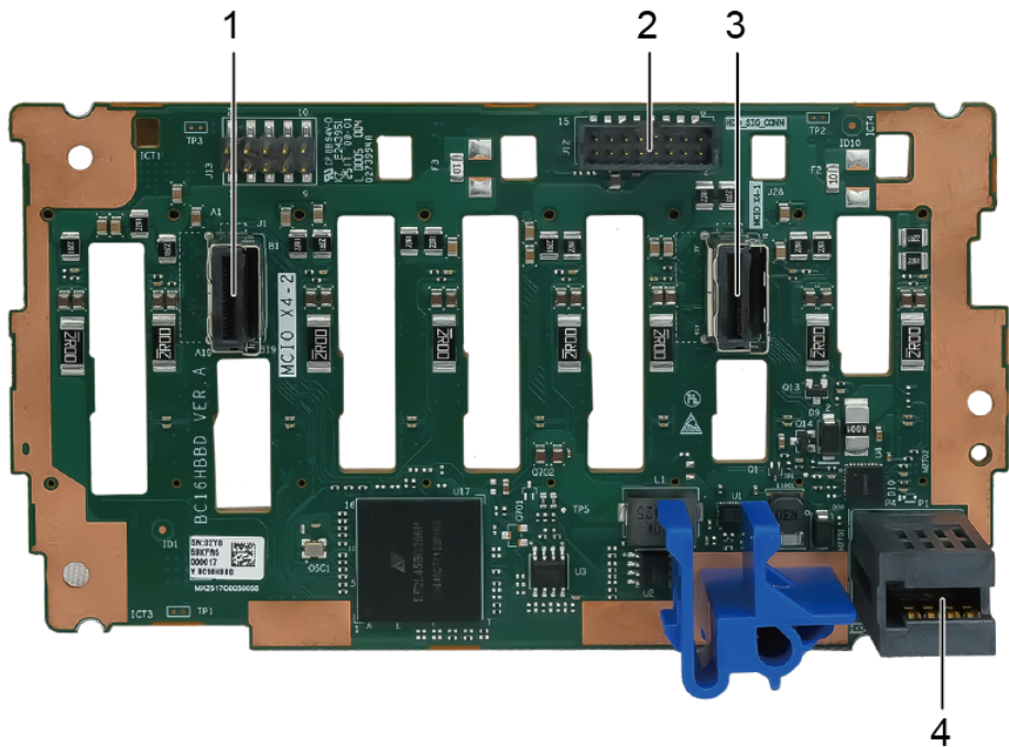
Figure 5-118 8 x 2.5" SAS/SATA 3cage drive backplane
