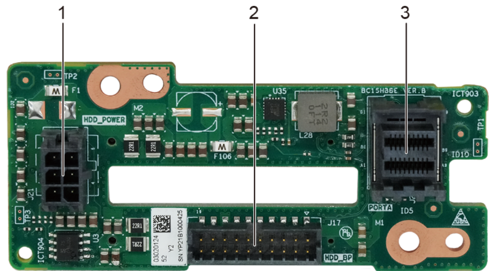
Figure 5-127 2 x 2.5" drive backplane
