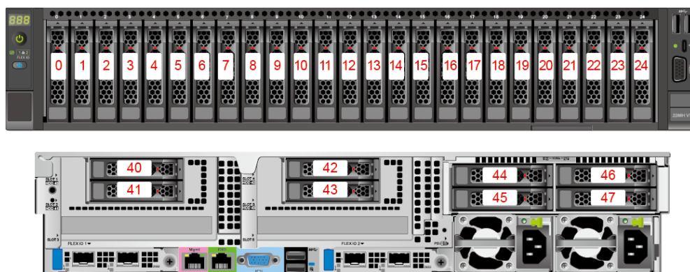
Figure 5-56 Drive numbers 1
