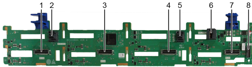
Figure 5-121 8 x 3.5" SAS/SATA/NVMe drive backplane
