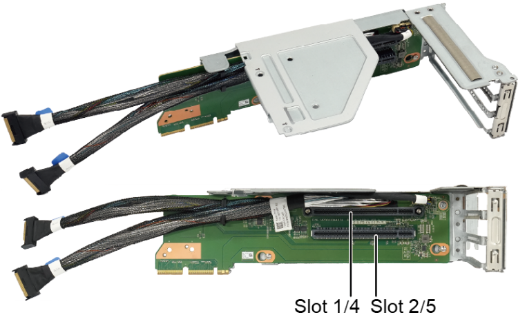
Figure 5-102 PCIe riser card 7 for IO module 1/I/O module 2 (BC16M01PRUI)
