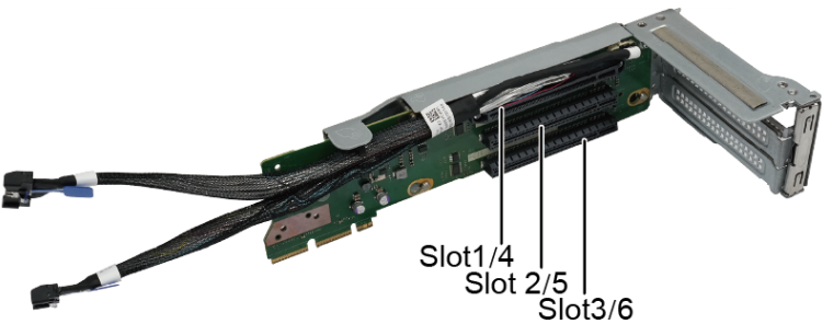
Figure 5-97 PCIe Riser card 2 (BC16M01PRUN)
