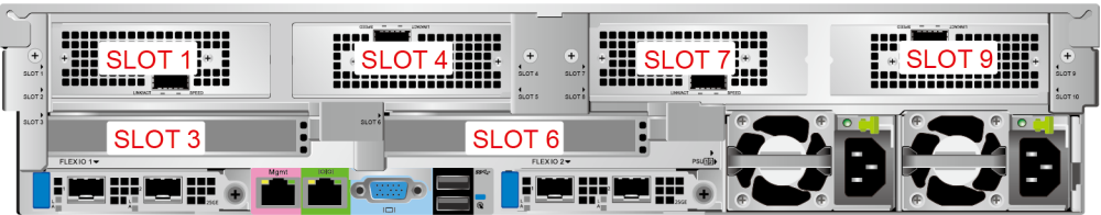
Figure 5-92 PCIe slots
