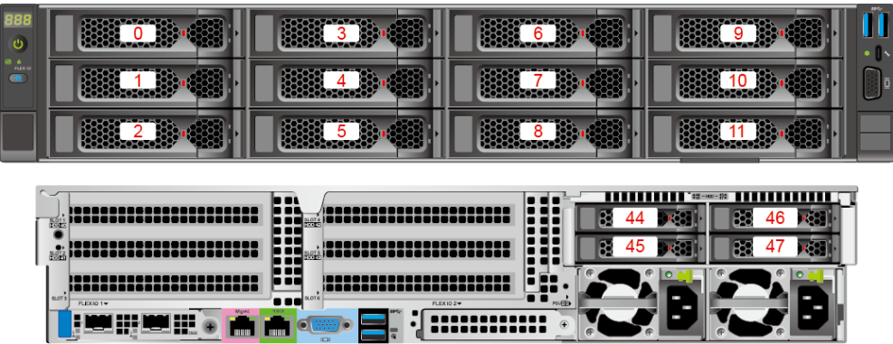
Figure 5-66 Drive numbers 1
