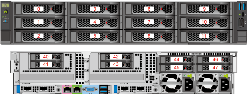
Figure 5-67 Drive numbers 1
