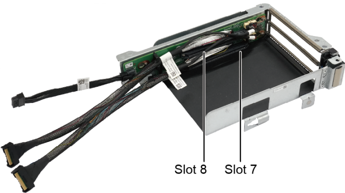
Figure 5-104 PCIe Riser card 1 of I/O module 3 (BC16M01PRUE)
