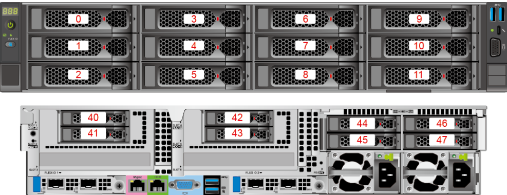
Figure 5-46 Drive numbers 1
