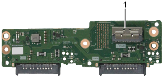
Figure 5-132 2 x 2.5" drive SAS/SATA/NVMe drive backplane 2
