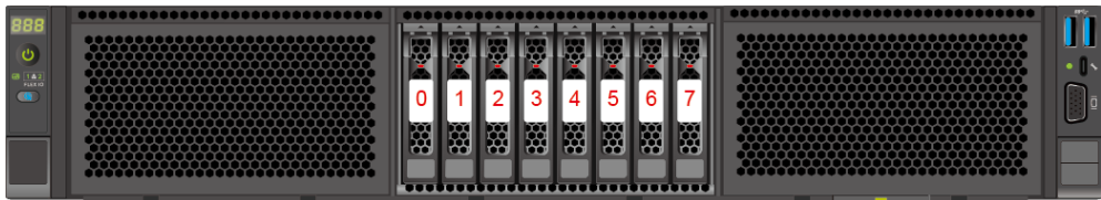
Figure 5-62 Drive numbers 1
