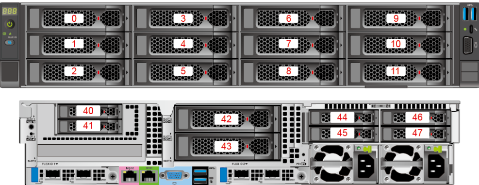
Figure 5-47 Drive number 2
