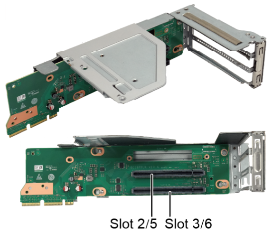
Figure 5-109 PCIe riser card 4 (BC16M02PRUKA - supports cable card)
