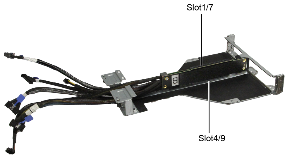
Figure 5-113 PCIe riser card 1 for rear GPU module (BC16M01PRHQ01)
