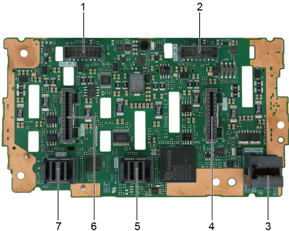
Figure 5-120 8 x 2.5" SAS/SATA/NVMe backplane (supporting hardware RAID)
