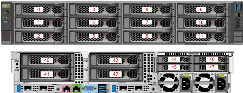
Figure 5-52 Drive numbers 4
