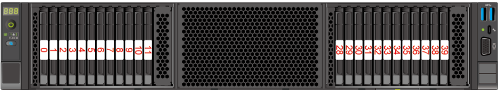
Figure 5-81 Drive numbers
