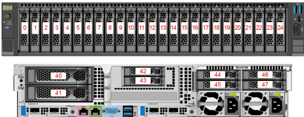
Figure 5-59 Drive numbers 4
