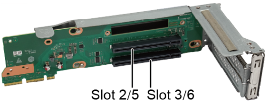
Figure 5-99 PCIe Riser card 4 (BC16M01PRUKA)
