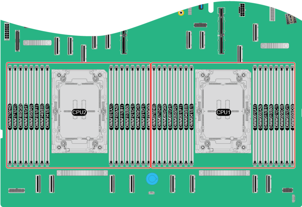
Figure 5-44 Positions of the memory modules
