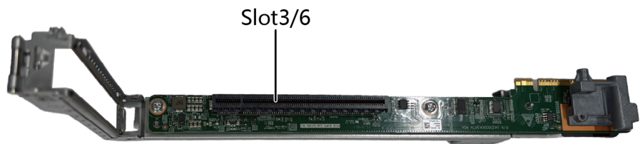
Figure 5-110 PCIe Riser card 4 of I/O module 1/2 (BC16M01PRUD)
