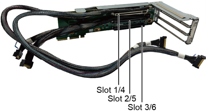
Figure 5-103 PCIe riser card 8 of I/O module 1/2 (BC16PRULA)
