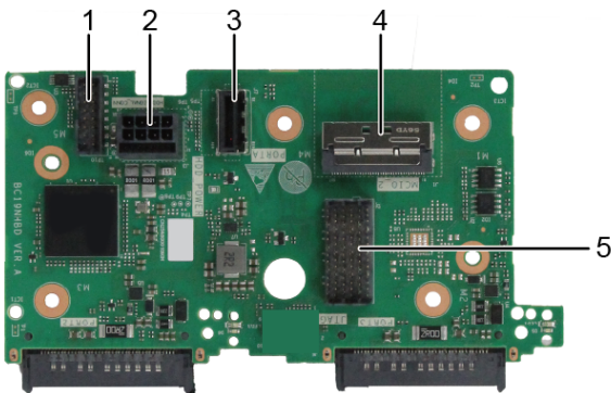
Figure 5-131 2 x 2.5" drive SAS/SATA/NVMe drive backplane 1
