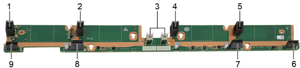
Figure 5-134 Fan board (P/N code: 0302012386)
