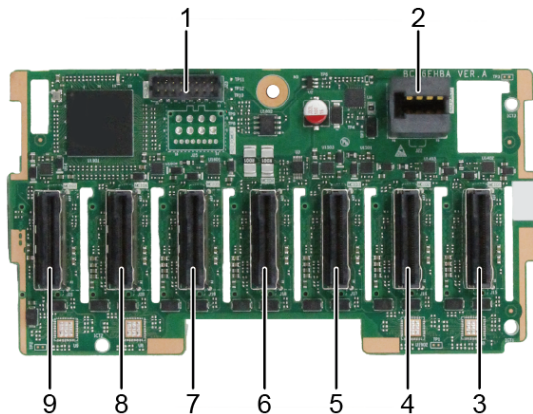
Figure 5-125 14 x E3.S 1 T NVMe 3Cage drive backplane
