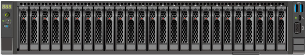
Figure 5-11 25 x 2.5" drive configuration
