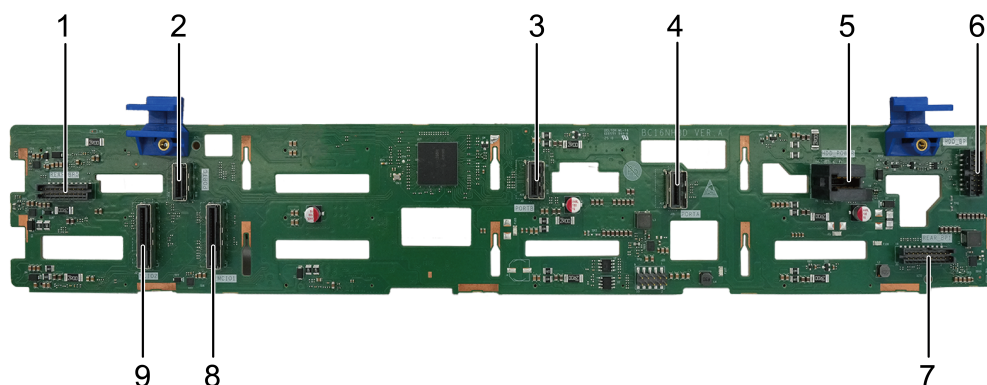
Figure 5-122 12 x 3.5" 8 x SAS/SATA + 4 x SAS/SATA/NVMe drive backplane
