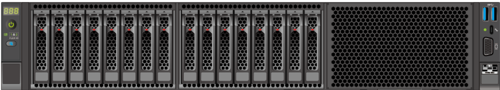
Figure 5-7 16 x 2.5" drive configuration 1
