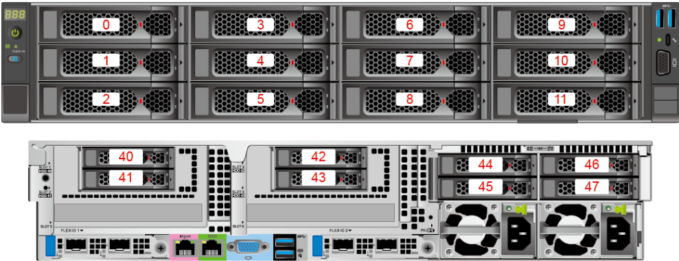
Figure 5-71 Drive numbers 1
