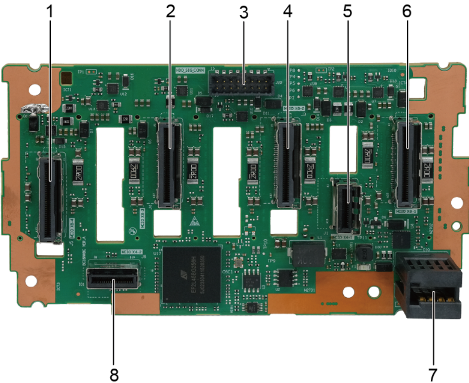
Figure 5-117 8 x 2.5" SAS/SATA/NVMe 3cage drive backplane
