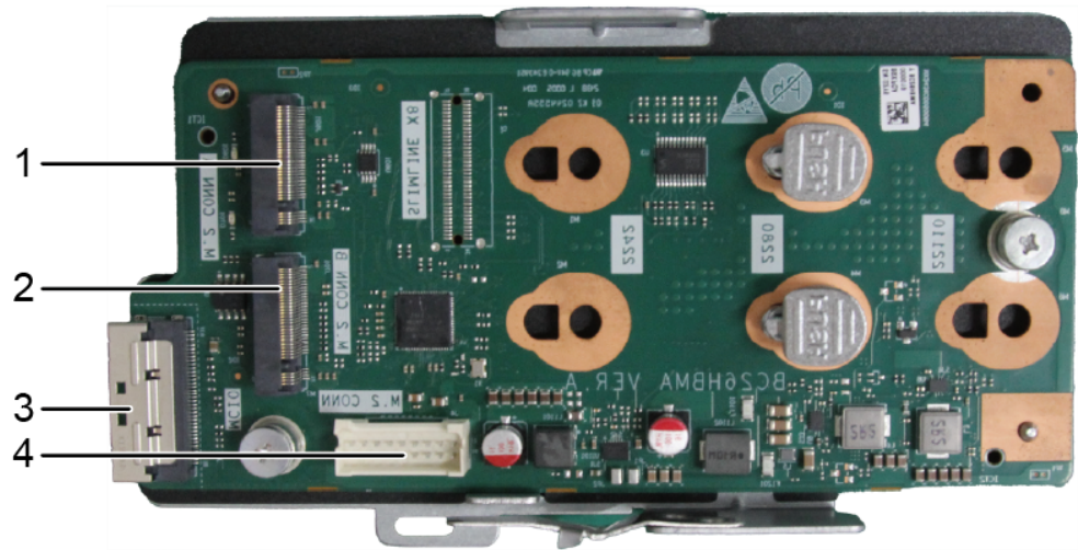
Figure 5-137 PCIe-SATA M.2 adapter card
