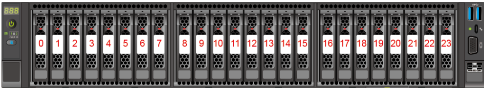
Figure 5-77 Drive numbers
