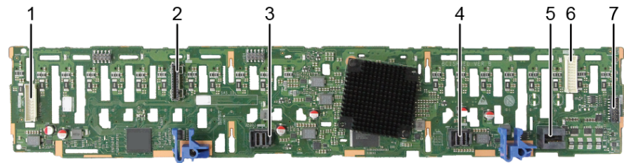
Figure 5-126 25 x 2.5" drive EXP backplane
