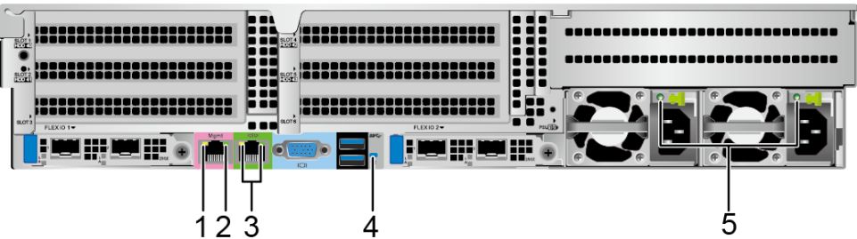
Figure 5-39 Indicators on the rear panel
