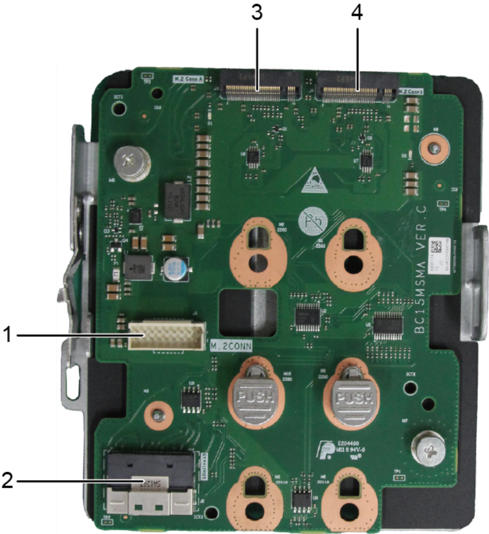
Figure 5-138 M.2 adapter card integrated in CPU
