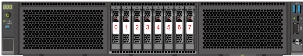
Figure 5-83 Drive numbers
