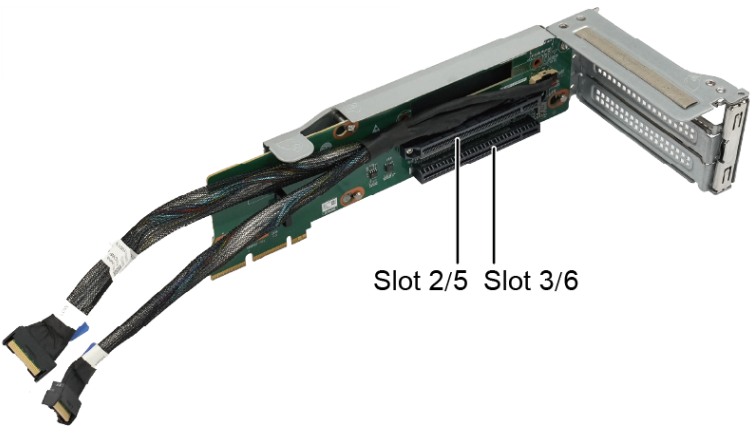
Figure 5-98 PCIe Riser card 3 (BC16M01PRUL)
