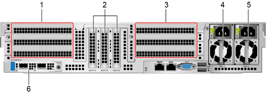
Figure 5-13 Rear view
