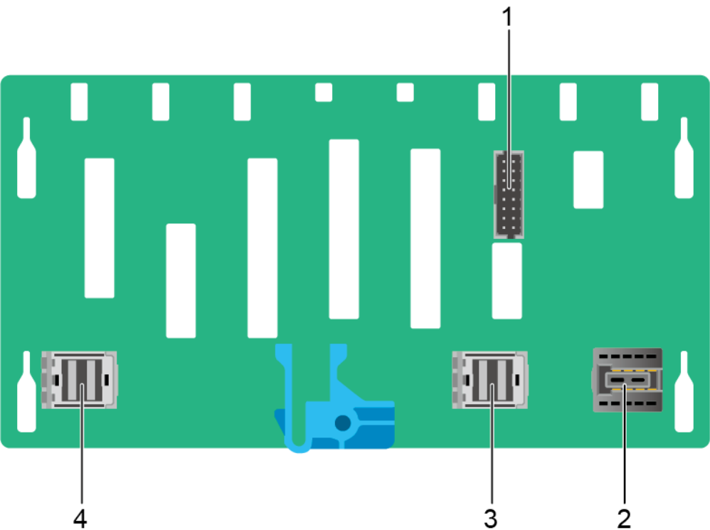
Figure 5-35 8 x 2.5" drive pass-through backplane
