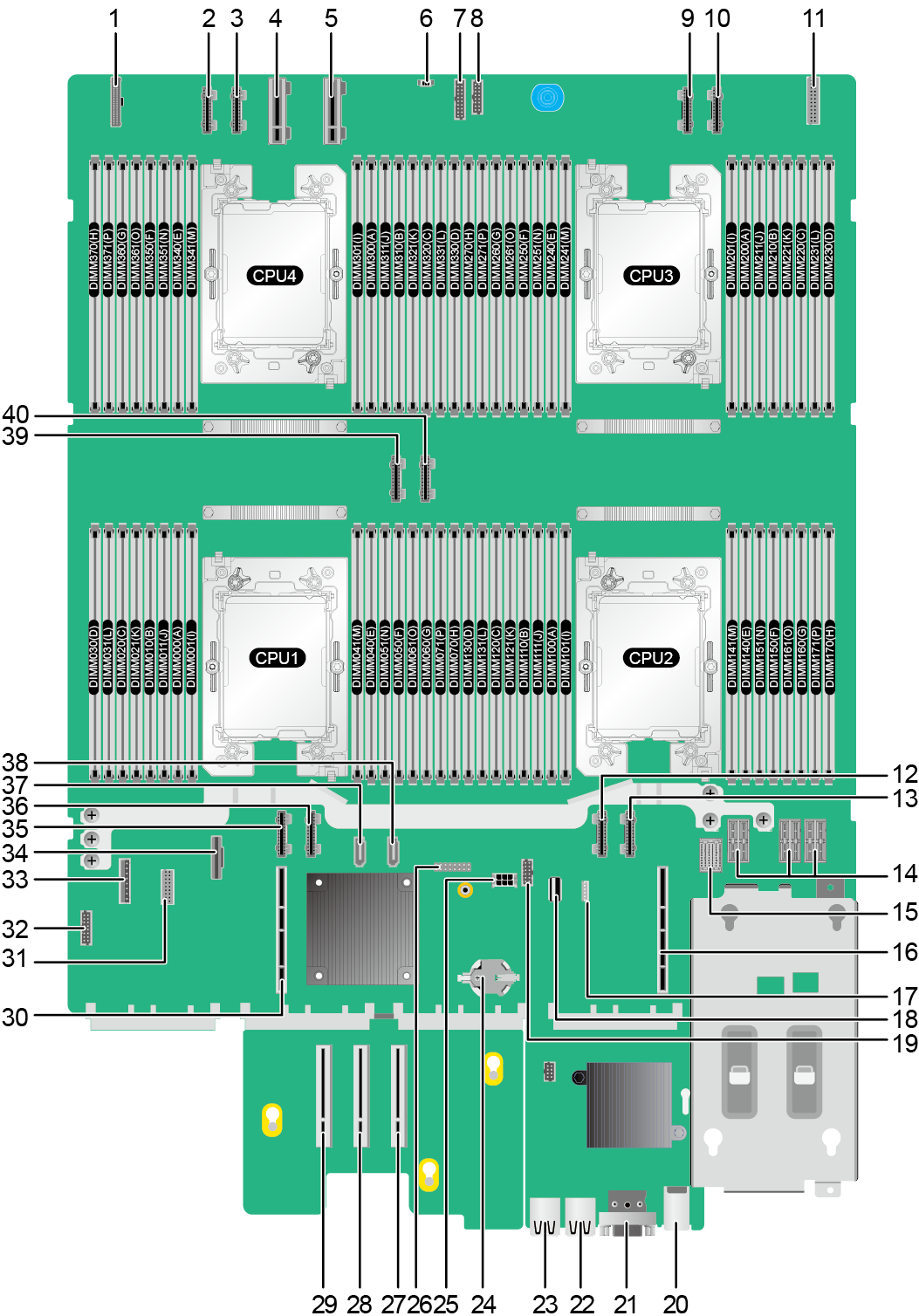
Figure 5-34 Mainboard
