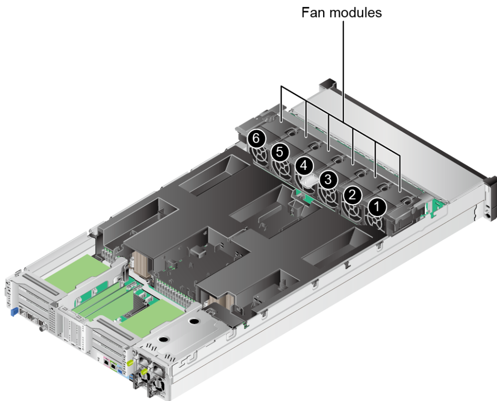
Figure 5-32 Positions of the fan modules
