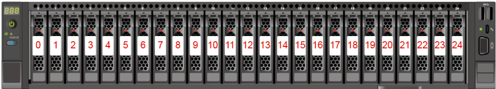
Figure 5-26 Drive numbering
