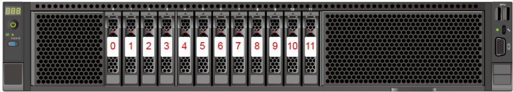
Figure 5-24 Drive numbering
