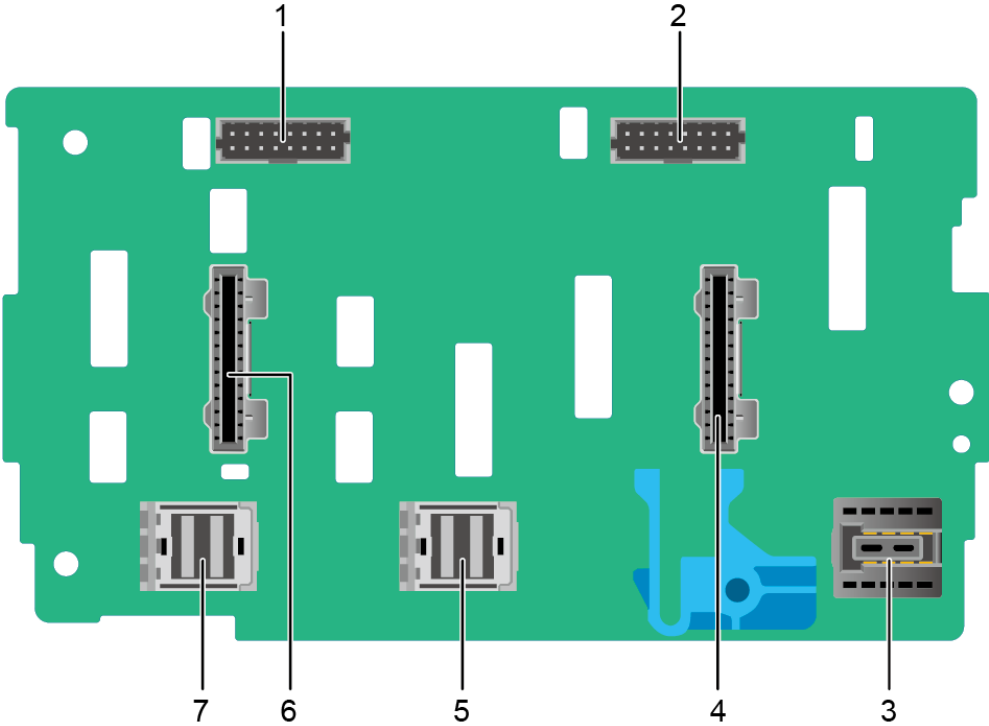
Figure 5-36 8 x 2.5" drives SAS/SATA/NVMe backplane (supporting hard RAID)
