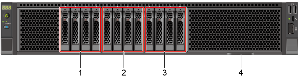
Figure 5-3 Front panel
