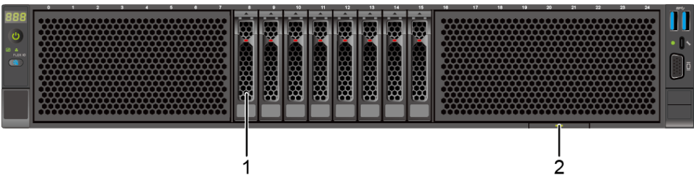
Figure 5-2 Front panel
