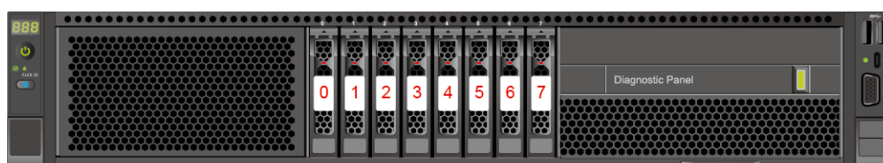
Figure 5-21 Drive Number
