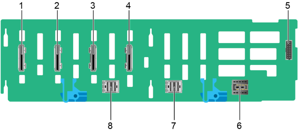
Figure 5-37 12 x 2.5" drive pass-through configuration backplane
