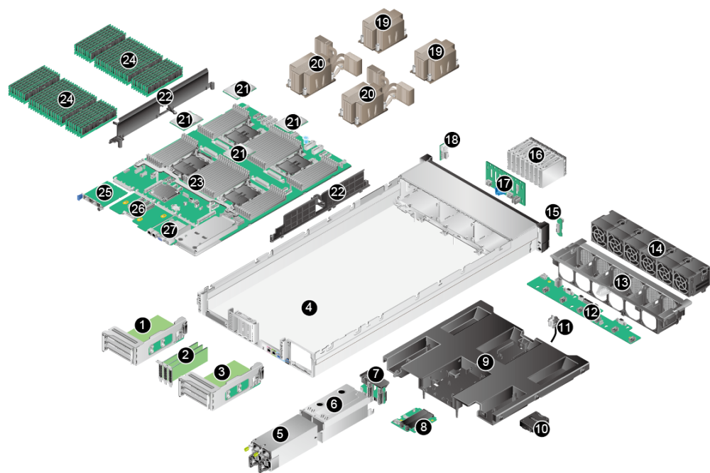
Figure 3-1 Physical structure of a server with 8 x 2.5" drives (example)
