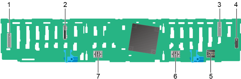
Figure 5-38 25 x 2.5" drive EXP backplane
