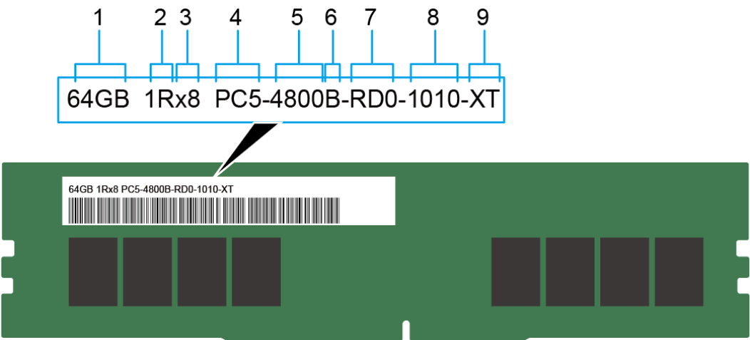
Figure 5-17 Memory identifier
