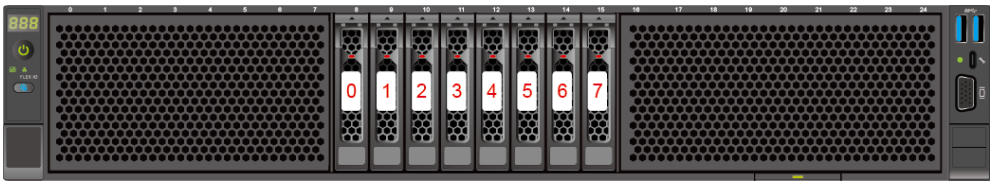
Figure 5-23 Drive Number
