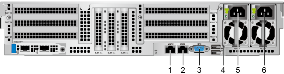
Figure 5-15 Ports on the rear panel
