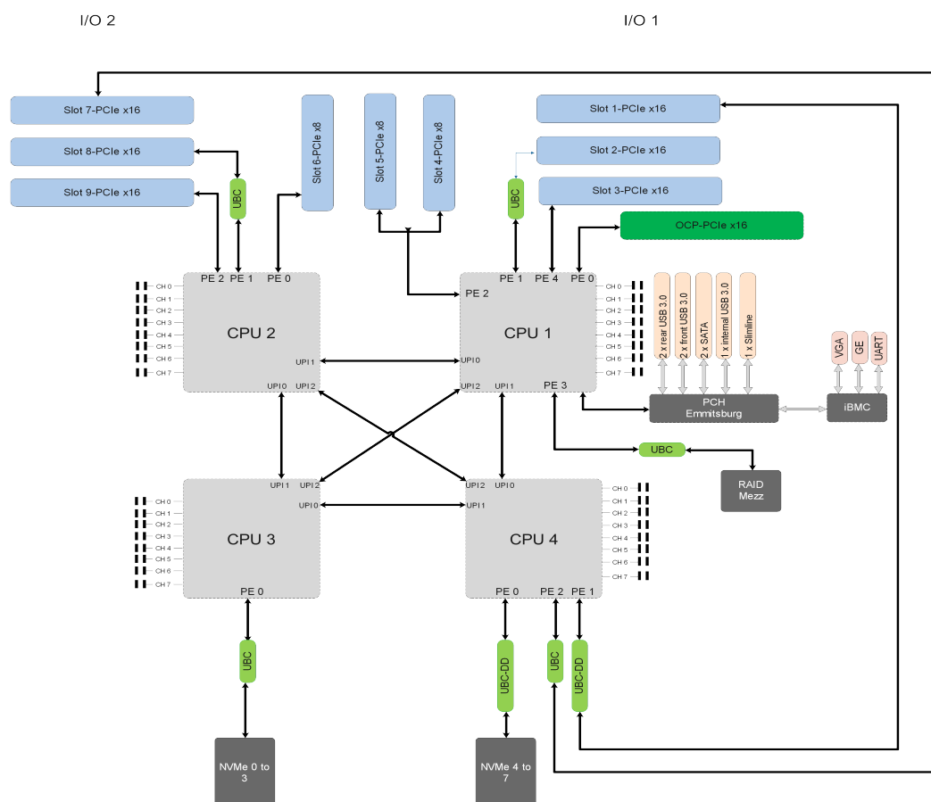
Figure 4-1 Logical Structure
