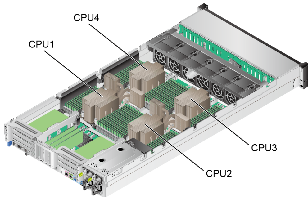
Figure 5-16 Positions of the processors
