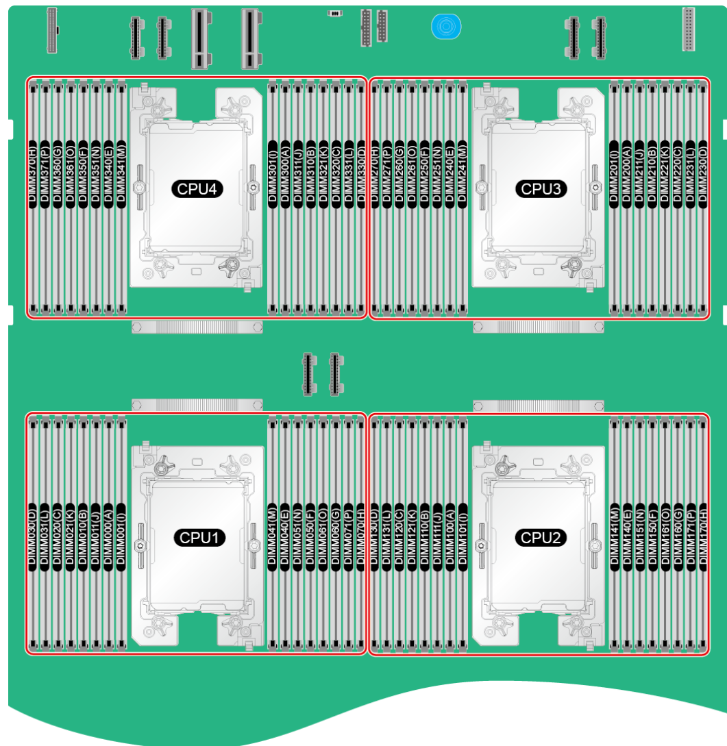
Figure 5-18 Positions of the memory modules
