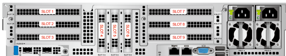
Figure 5-29 PCIe slots
