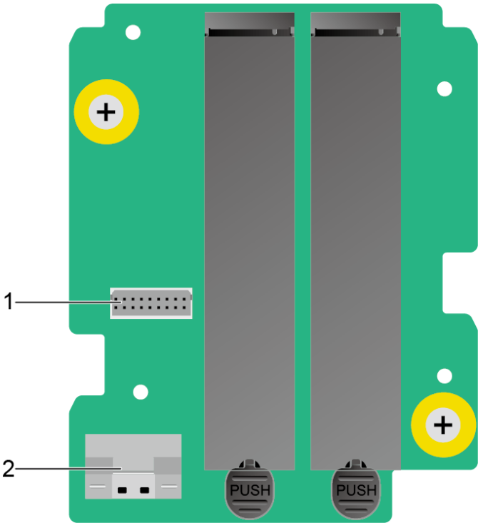
Figure 5-41 M.2 SSD adapter board
