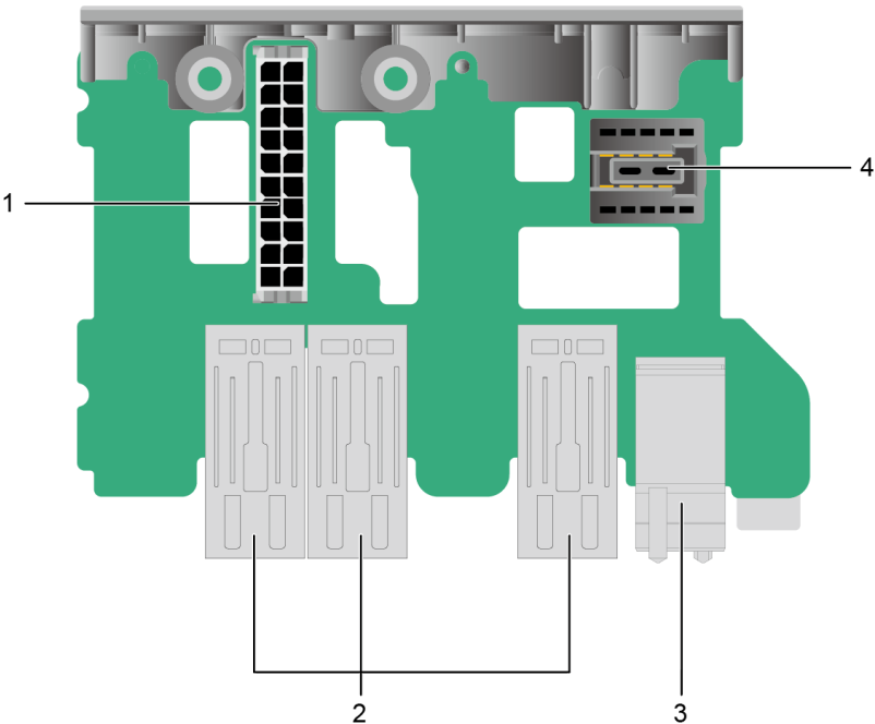
Figure 5-39 PSU Backplane
