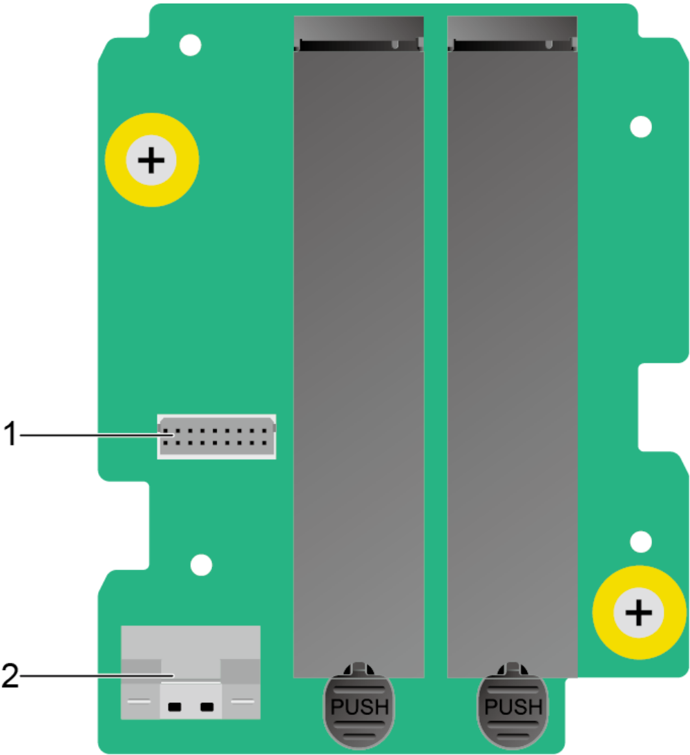
Figure 5-47 M.2 adapter board
