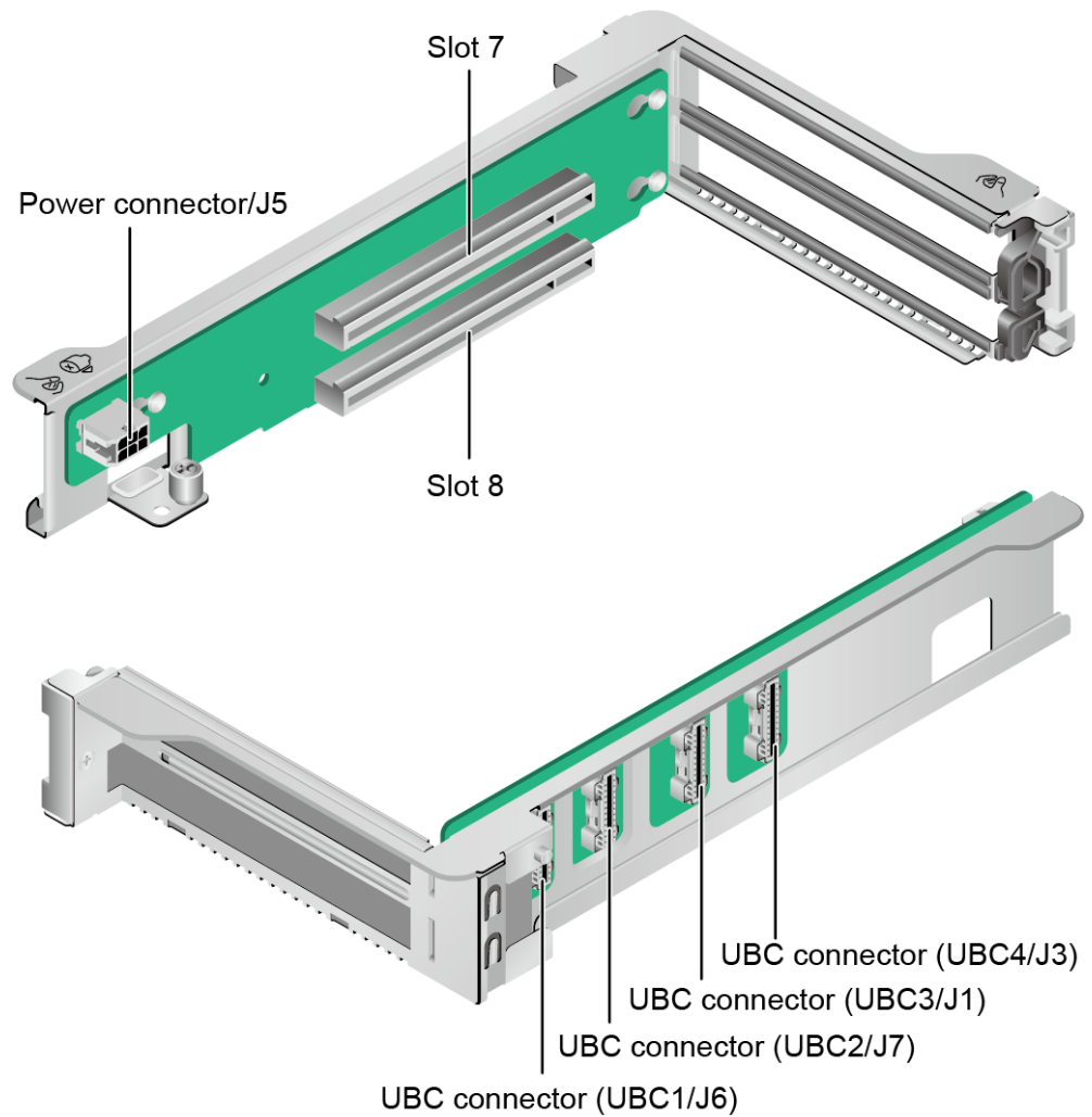
Figure 5-32 PCIe riser card 1
