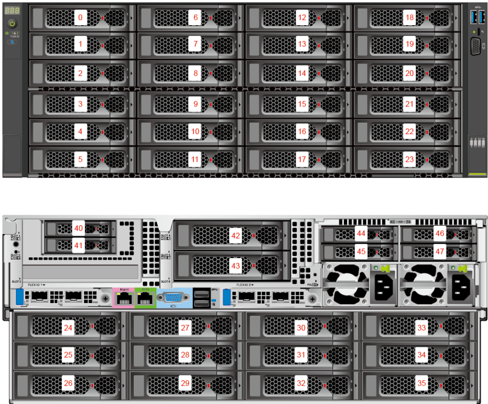
Figure 5-17 Drive numbering (I/O module 1 configured with 2.5" drives + I/O module 2 configured with 3.5" drives + I/O module 3 configured with NVMe drives)
