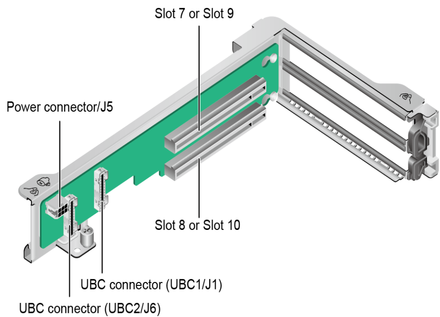
Figure 5-33 PCIe riser card 2
