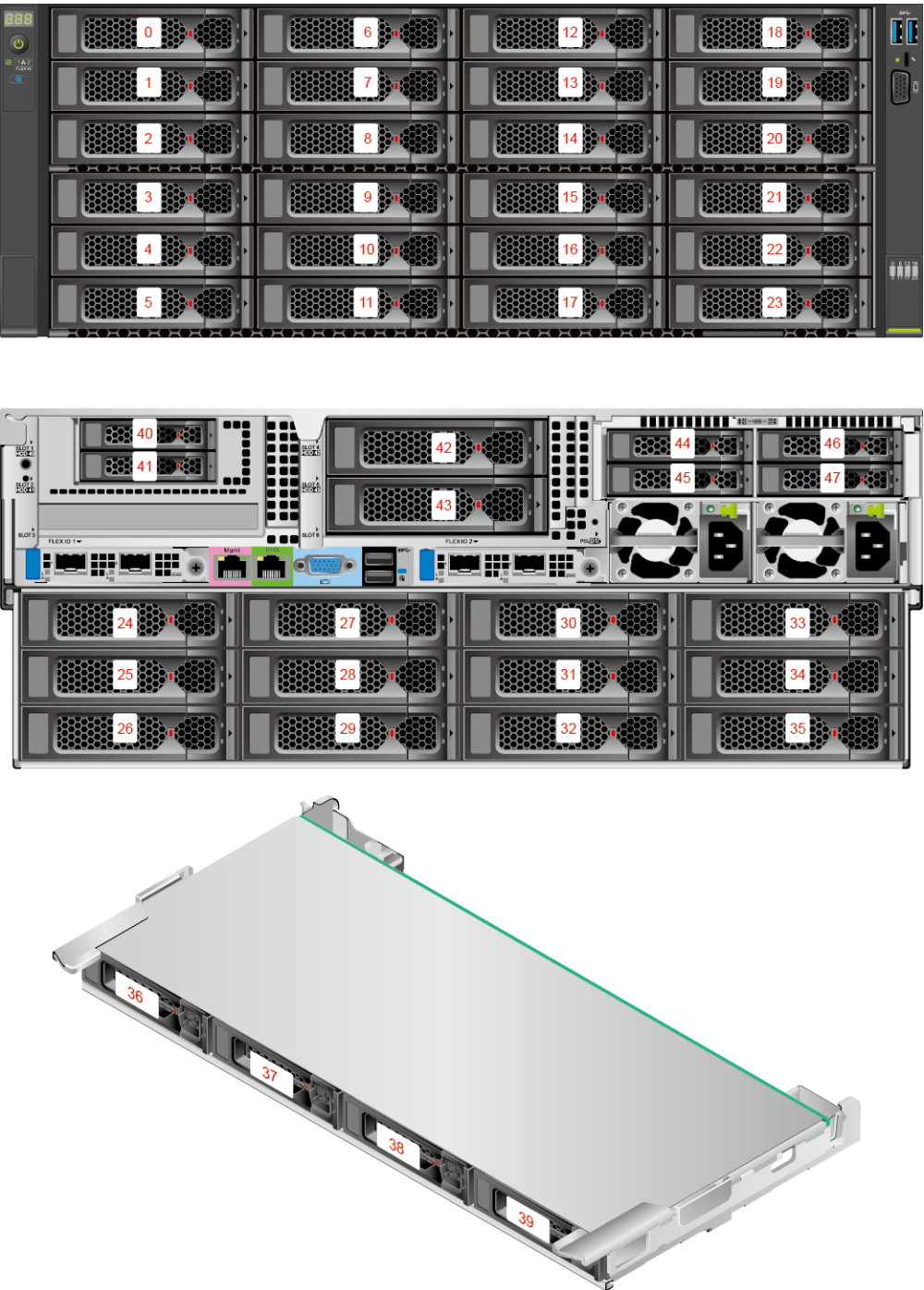
Figure 5-19 Drive numbering (I/O module 1 configured with 2.5" drives + I/O module 2 configured with 3.5" drives + I/O module 3 configured with NVMe/SAS/SATA drives)
