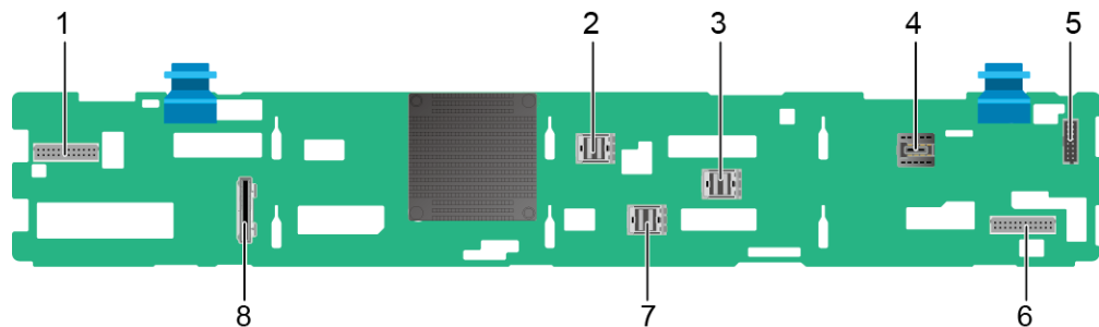
Figure 5-44 12 x 3.5" drive EXP backplane
