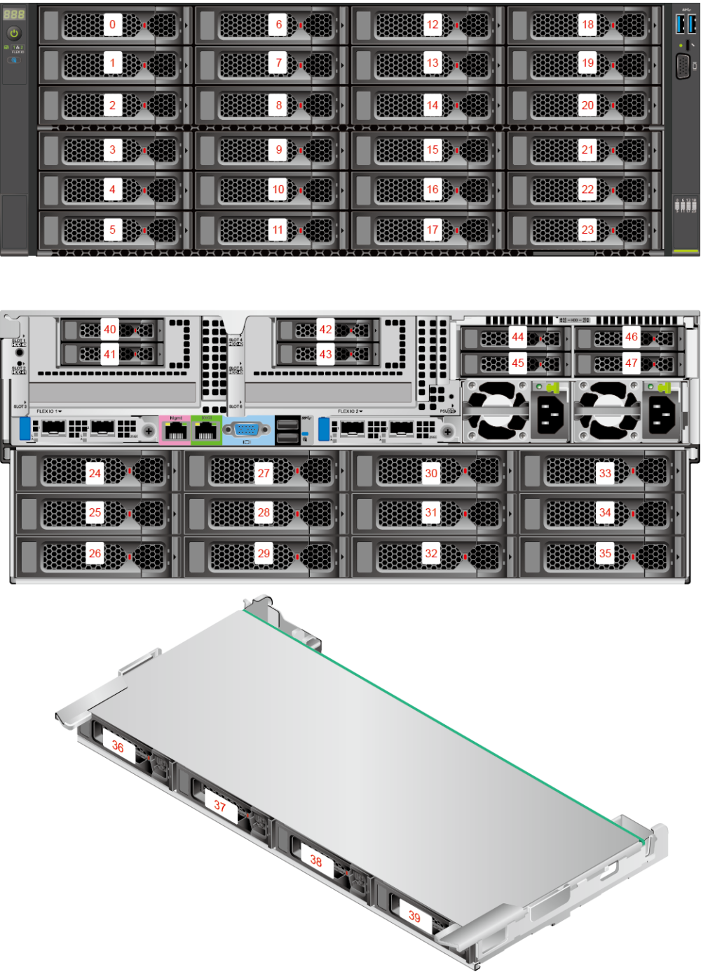
Figure 5-23 Drive numbering (I/O module 1 configured with 2.5" drives + I/O module 2 configured with 2.5" drives + I/O module 3 configured with NVMe/SAS/SATA drives)
