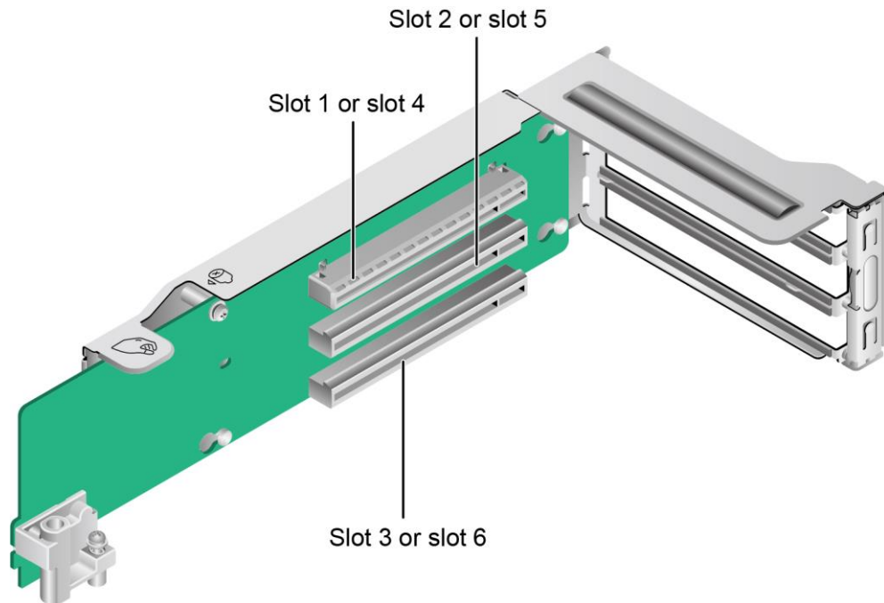
Figure 5-29 PCIe riser card 1
