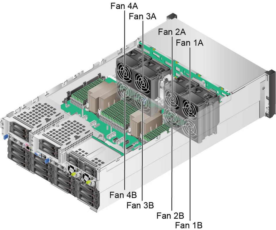
Figure 5-35 Positions of the fan modules
