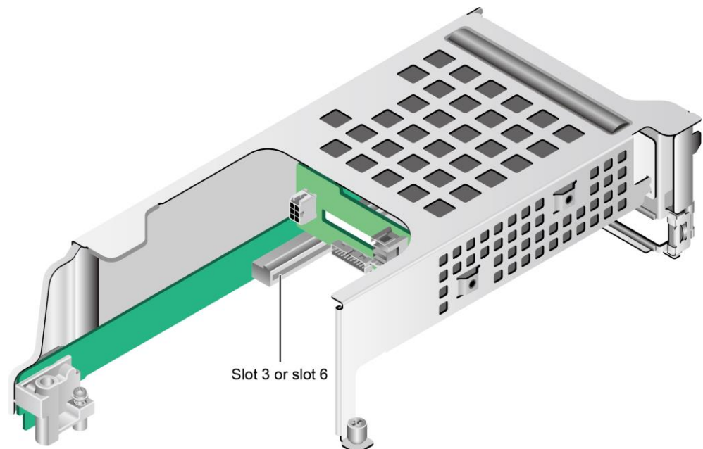
Figure 5-30 PCIe riser card 2
