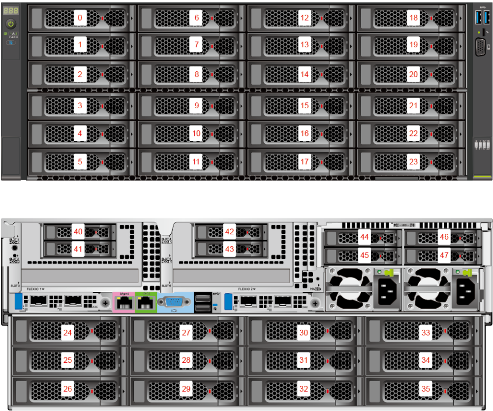
Figure 5-16 Drive numbering (I/O module 1 configured with 2.5" drives + I/O module 2 configured with 2.5" drives + I/O module 3 configured with NVMe drives)
