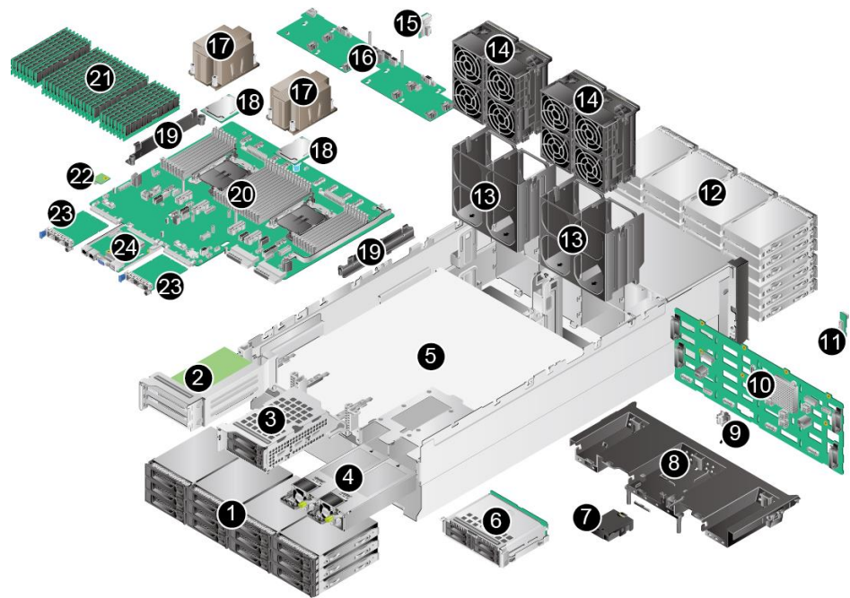
Figure 3-1 Physical structure
