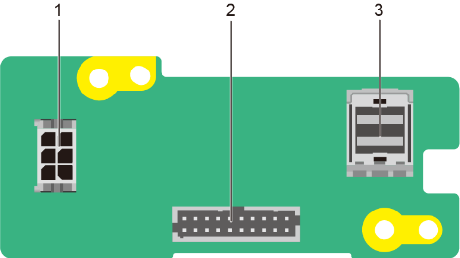
Figure 5-39 2 x 2.5" drive backplane
