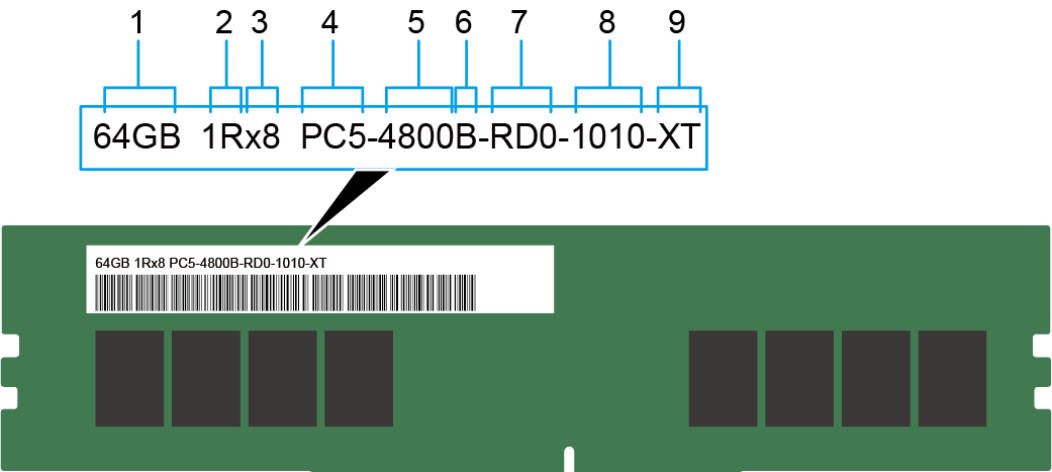
Figure 5-8 Memory identifier
