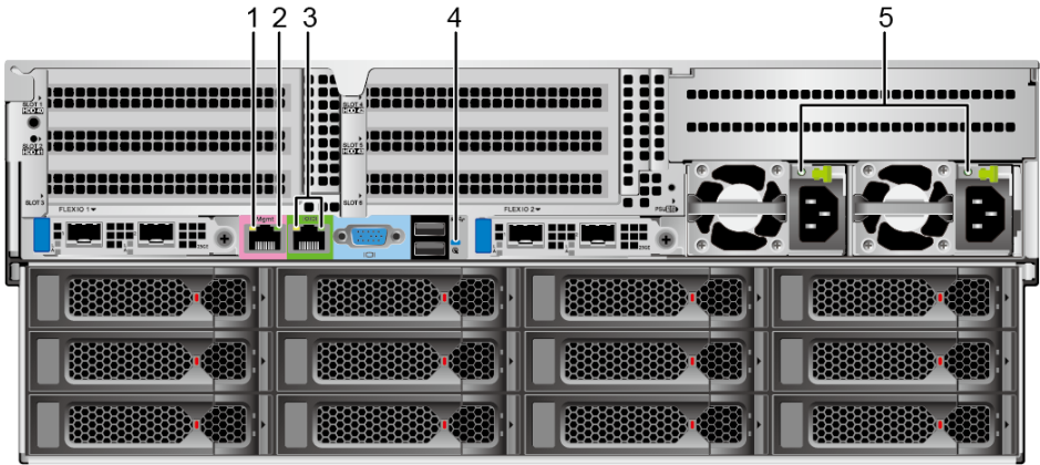
Figure 5-5 Indicators on the rear panel
