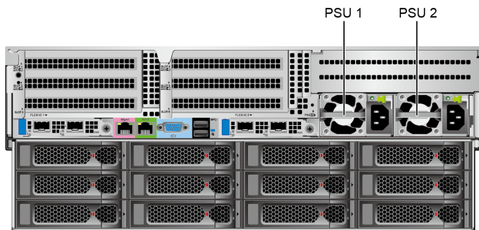
Figure 5-34 Positions of PSUs
