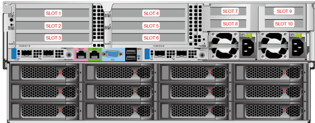
Figure 5-28 PCIe slots
