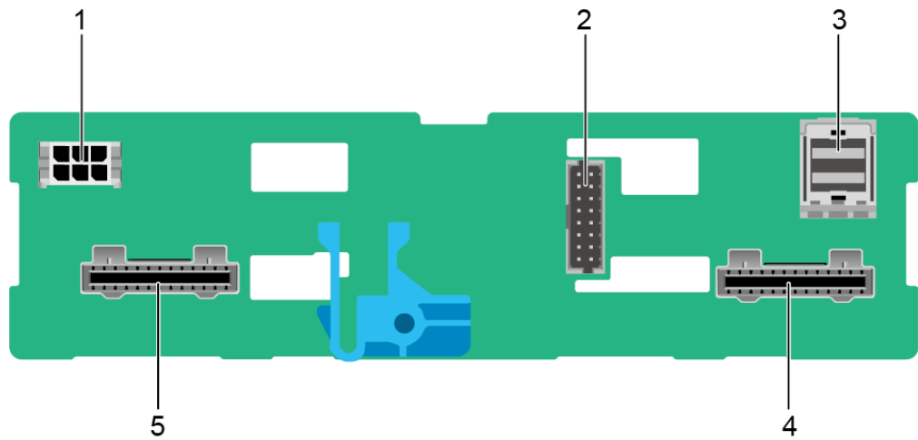
Figure 5-41 4 x 2.5" drive backplane
