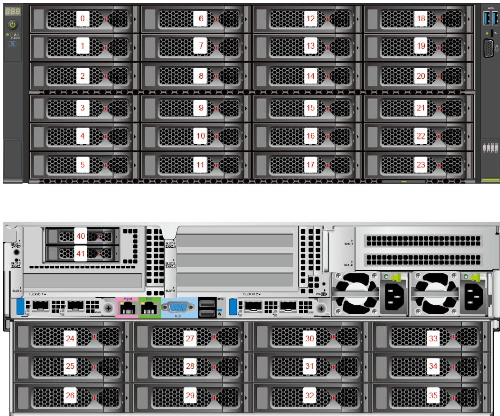
Figure 5-20 Drive numbering
