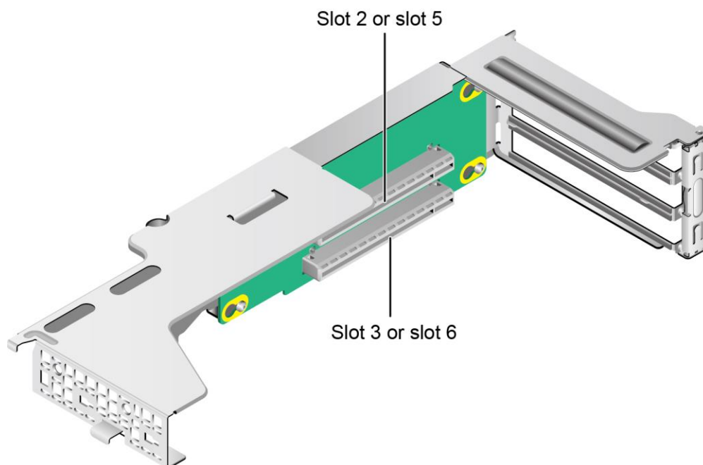
Figure 5-31 PCIe riser card 3
