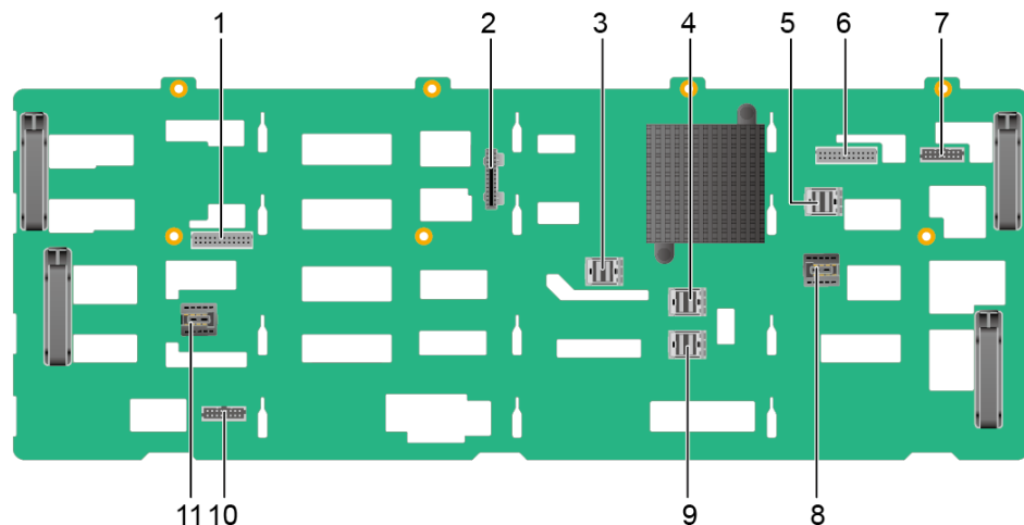
Figure 5-37 24 x 3.5" drive EXP backplane
