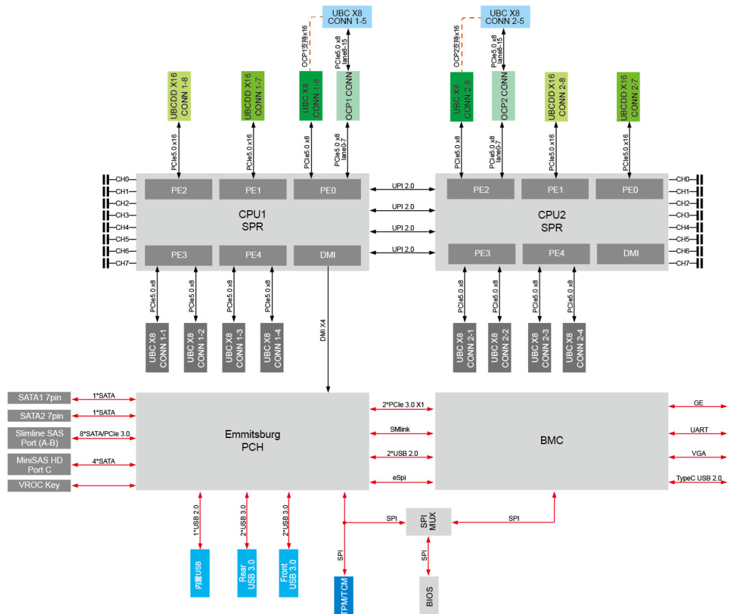
Figure 4-1 Logic structure
