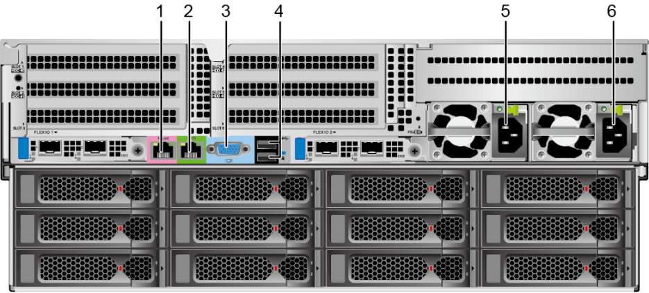
Figure 5-6 Ports on the rear panel
