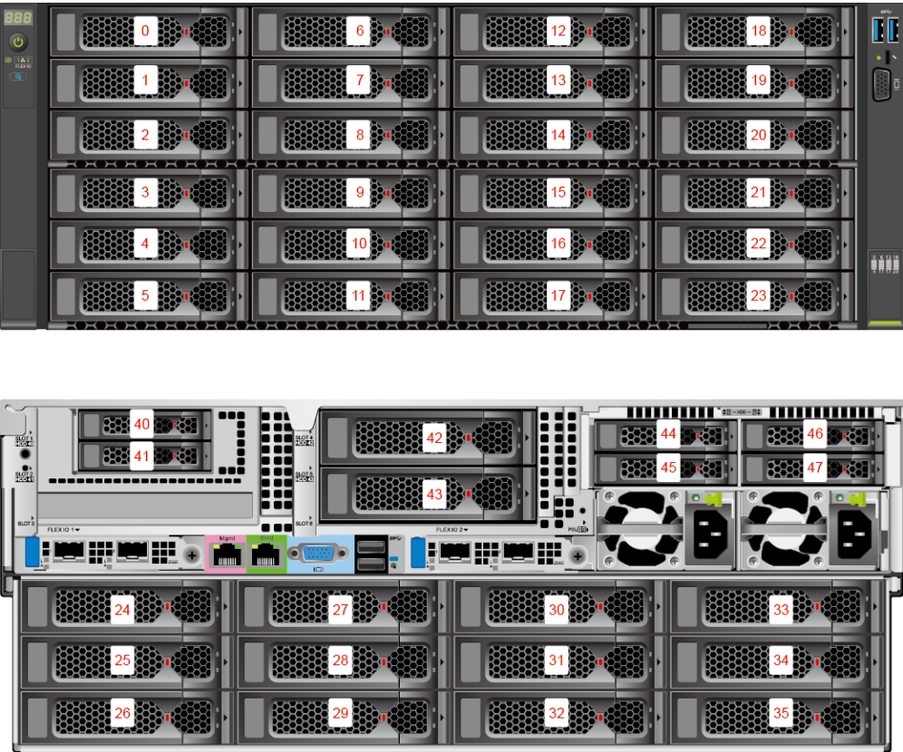
Figure 5-22 Drive numbering (I/O module 1 configured with 2.5" drives + I/O module 2 configured with 3.5" drives + I/O module 3 configured with NVMe drives)
