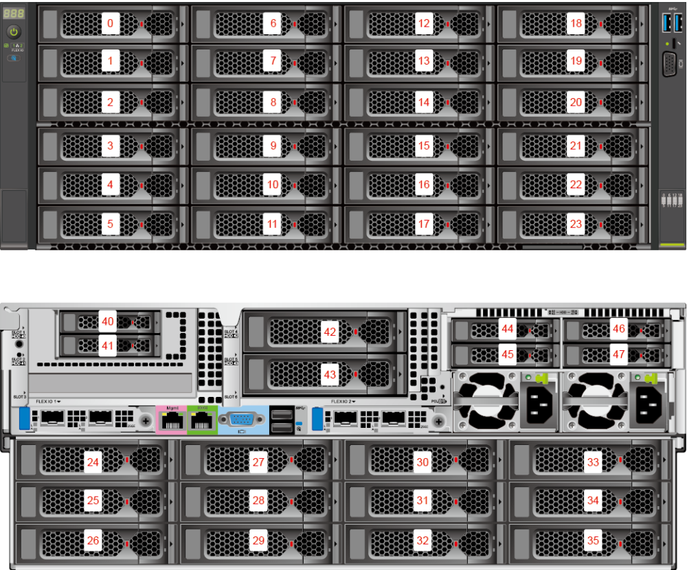
Figure 5-13 Drive numbering (I/O module 1 configured with 2.5" drives + I/O module 2 configured with 3.5" drives + I/O module 3 configured with NVMe drives)
