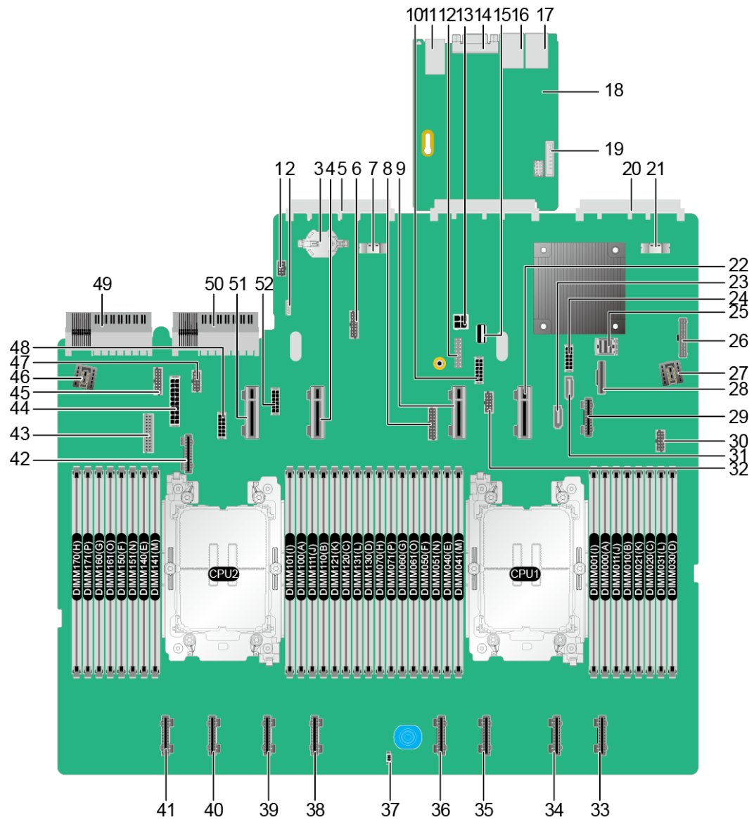
Figure 5-36 Mainboard
