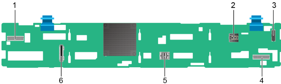
Figure 5-45 12 x 3.5" drive EXP backplane 2
