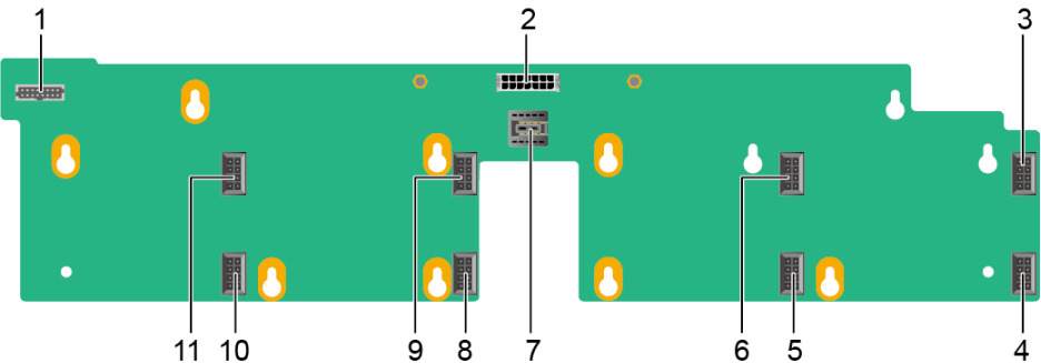
Figure 5-46 Fan board
