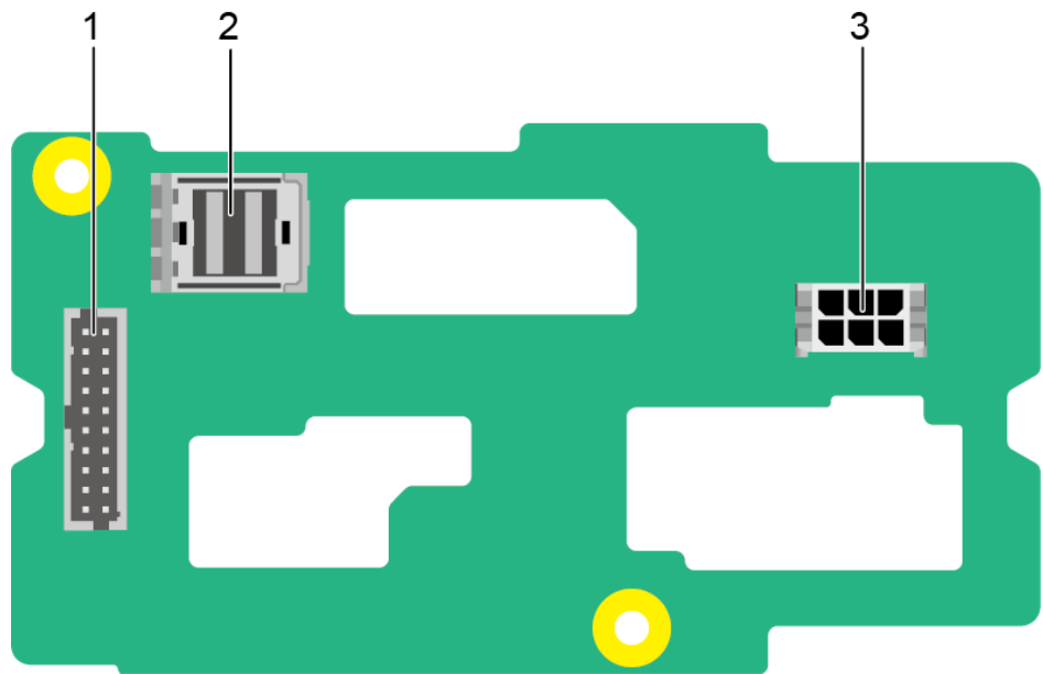
Figure 5-40 2 x 3.5" drive backplane
