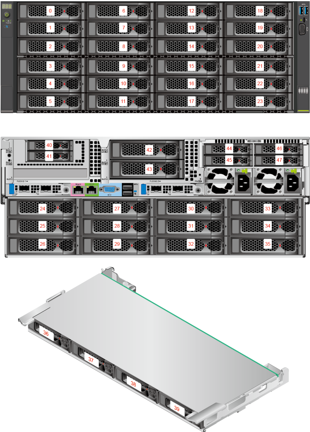
Figure 5-24 Drive numbering (I/O module 1 configured with 2.5" drives + I/O module 2 configured with 3.5" drives + I/O module 3 configured with NVMe/SAS/SATA drives)
