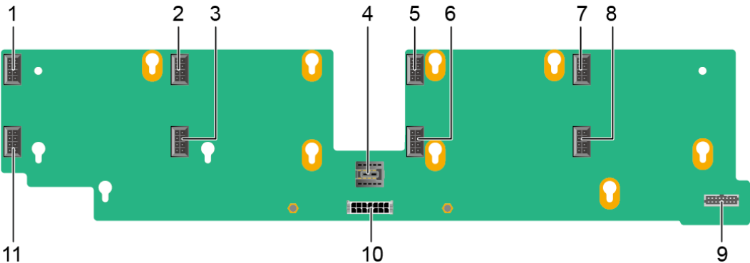
Figure 5-67 Fan board 1
