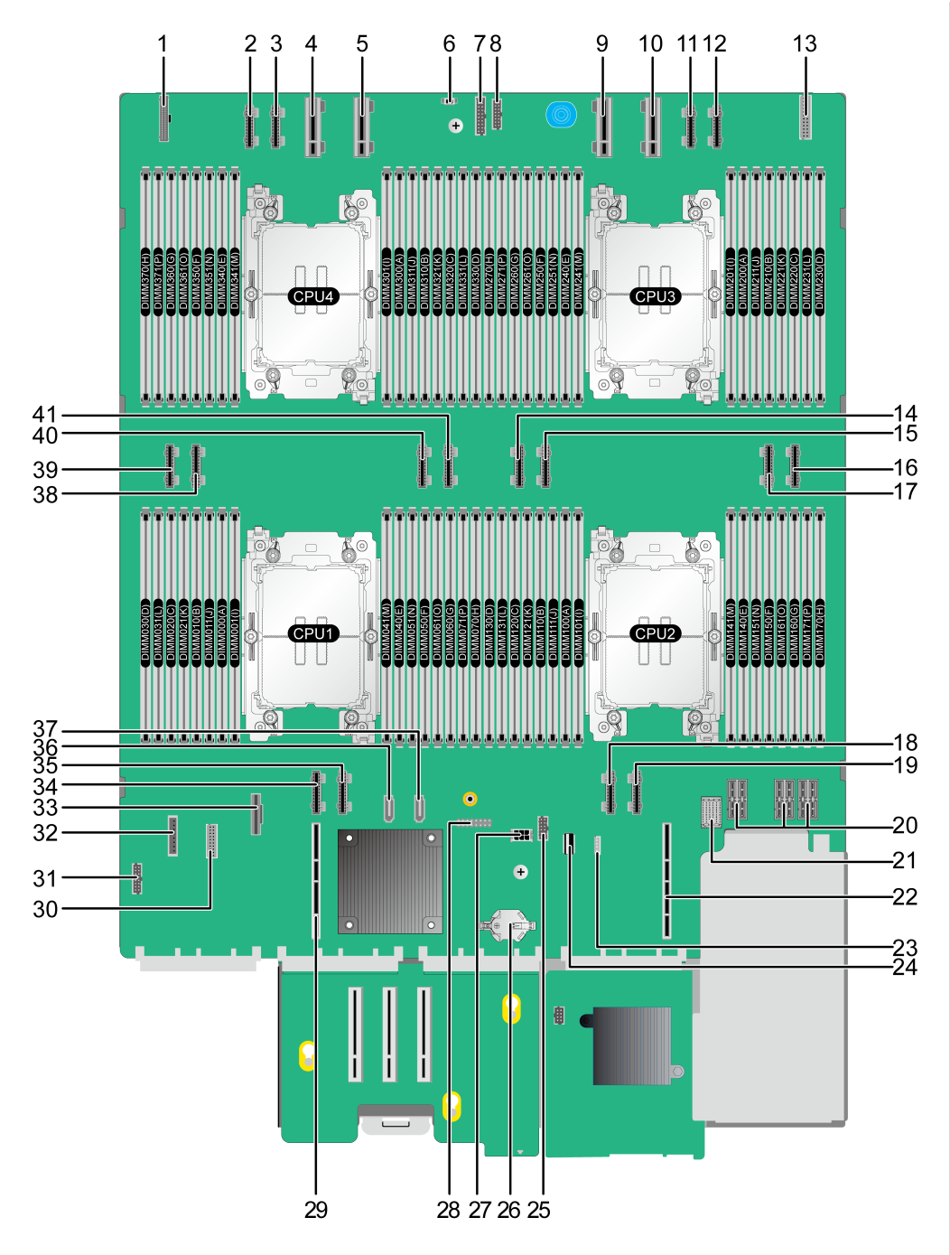
Figure 5-58 Mainboard
