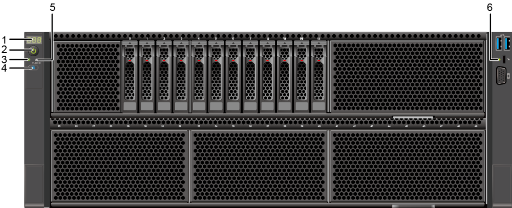
Figure 5-9 Indicators and buttons on the front panel
