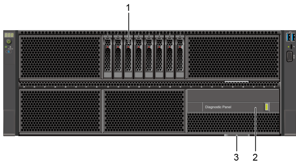
Figure 5-1 Front view
