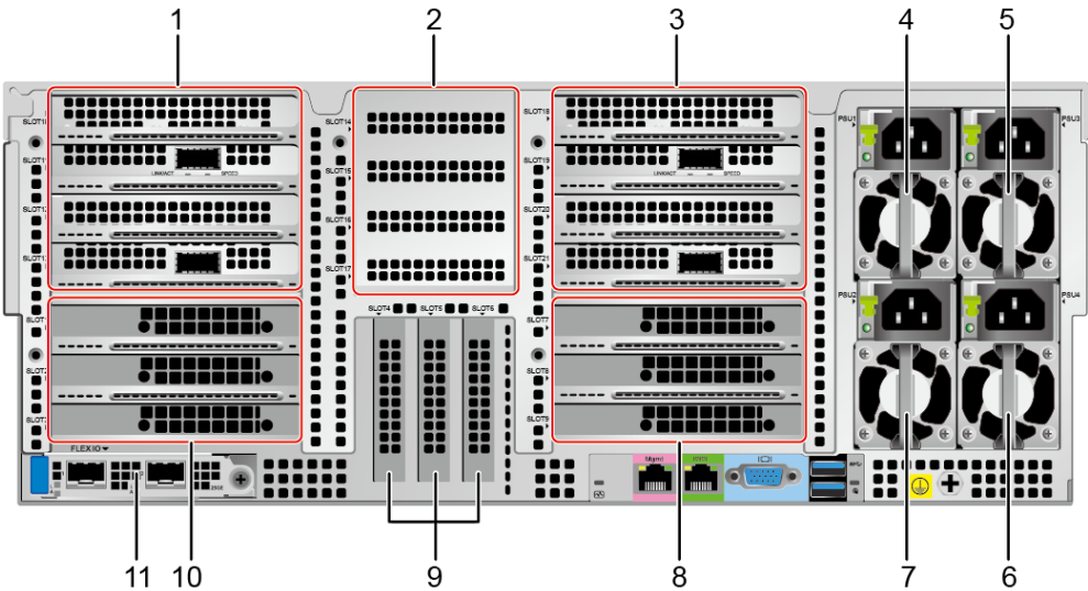
Figure 5-23 Rear view
