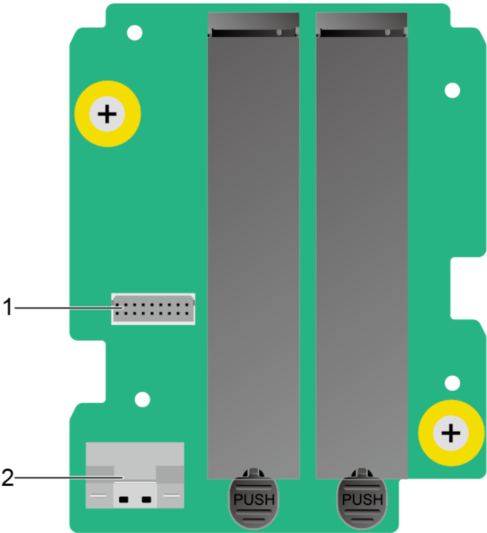
Figure 5-68 M.2 SSD adapter board
