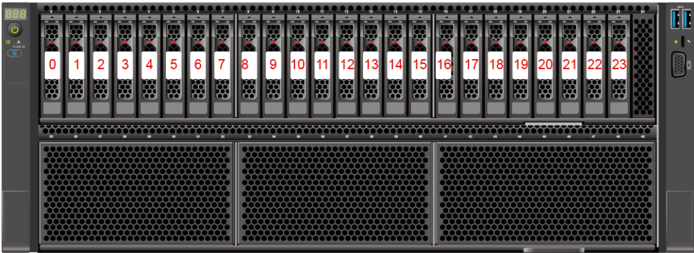
Figure 5-45 Drive numbering
