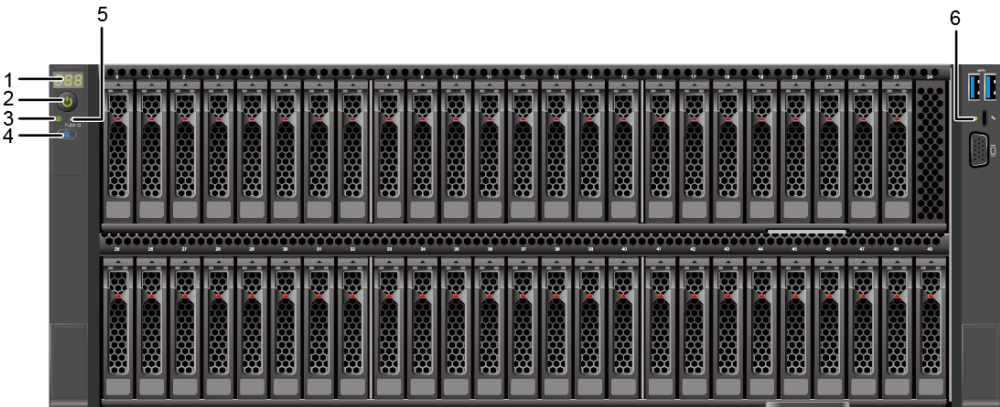
Figure 5-13 Indicators and buttons on the front panel
