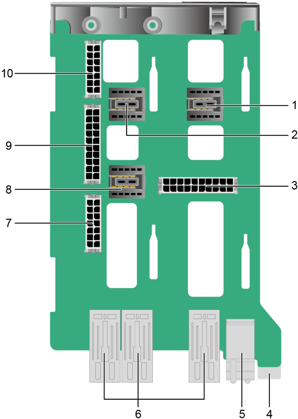
Figure 5-66 PSU backplane
