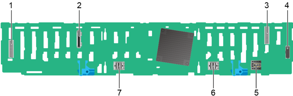
Figure 5-63 25 x 2.5" drive EXP backplane
