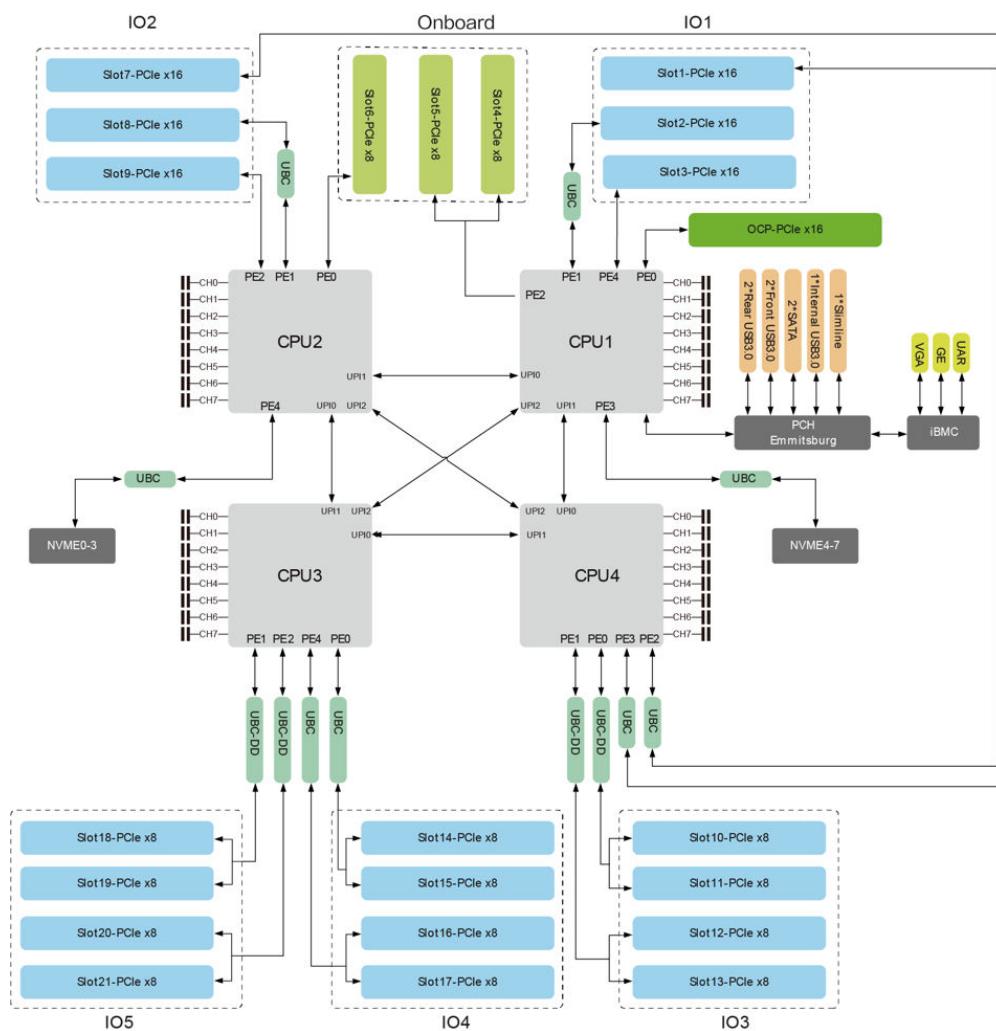
Figure 4-1 Logic structure
