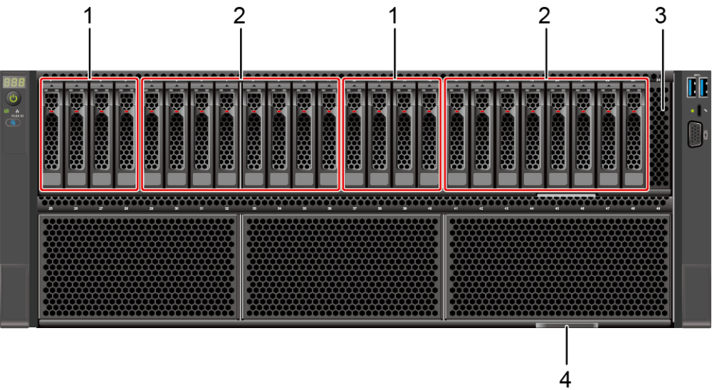
Figure 5-5 Front view
