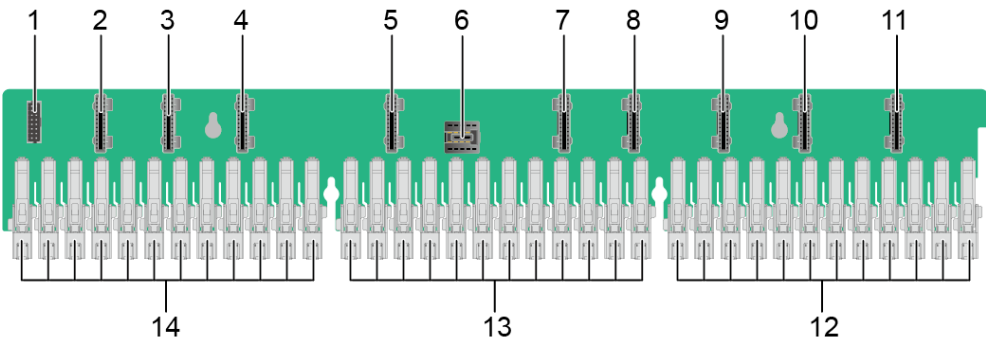
Figure 5-64 E1.S drive pass-through backplane
