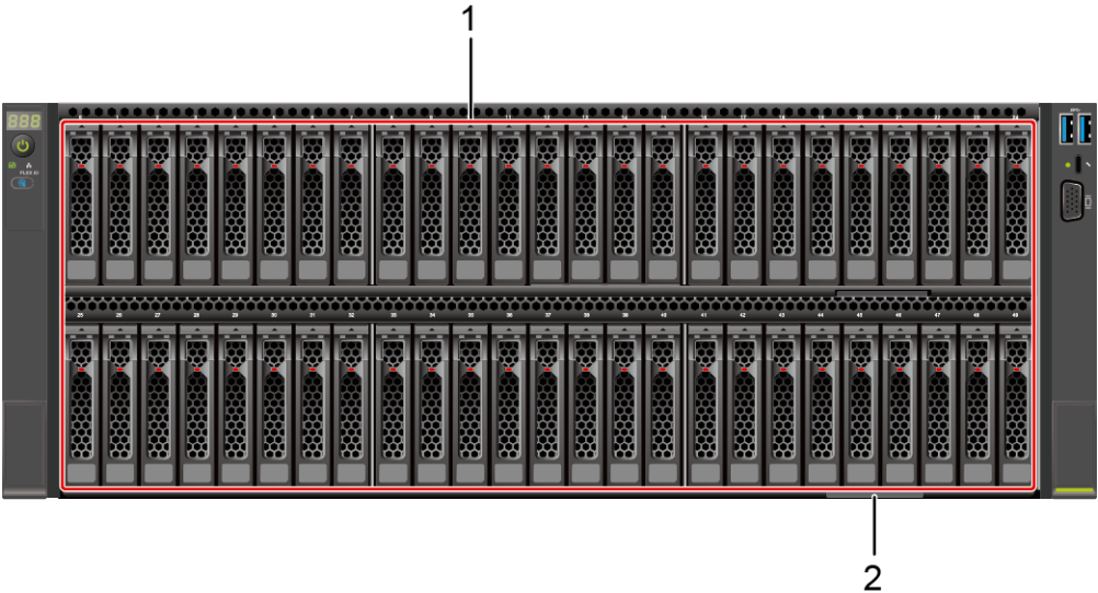
Figure 5-7 Front view
