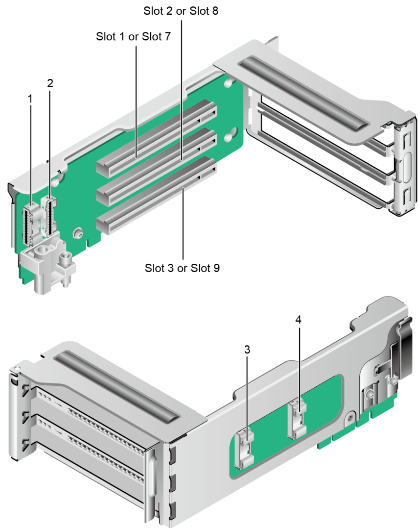
Figure 5-52 PCIe riser card 1
