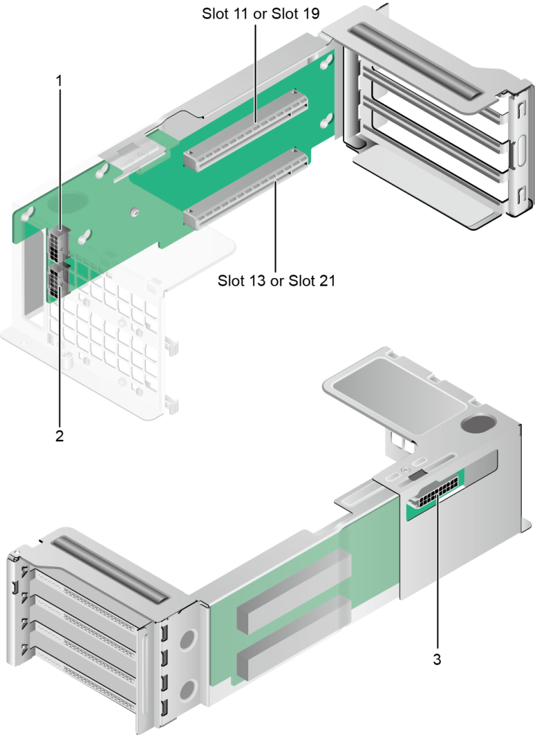
Figure 5-54 PCIe riser card 3 (supporting GPU cards)
