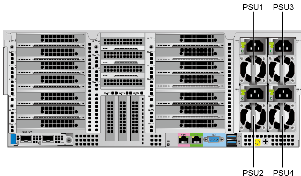
Figure 5-55 Positions of PSUs
