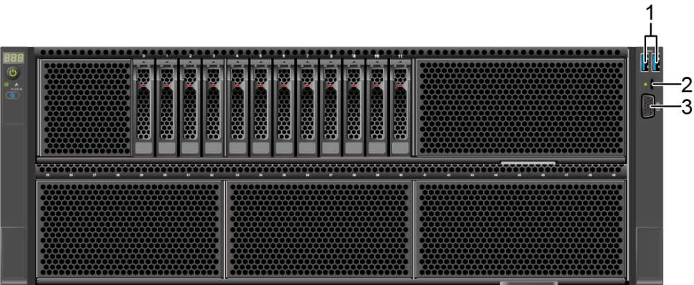
Figure 5-16 Ports on the front panel
