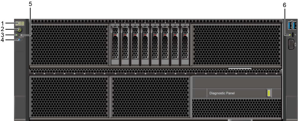
Figure 5-8 Indicators and buttons on the front panel
