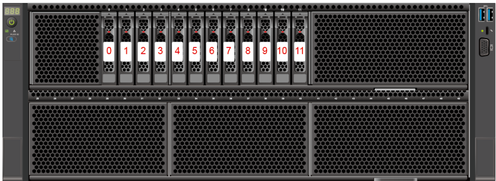
Figure 5-39 Drive numbering
