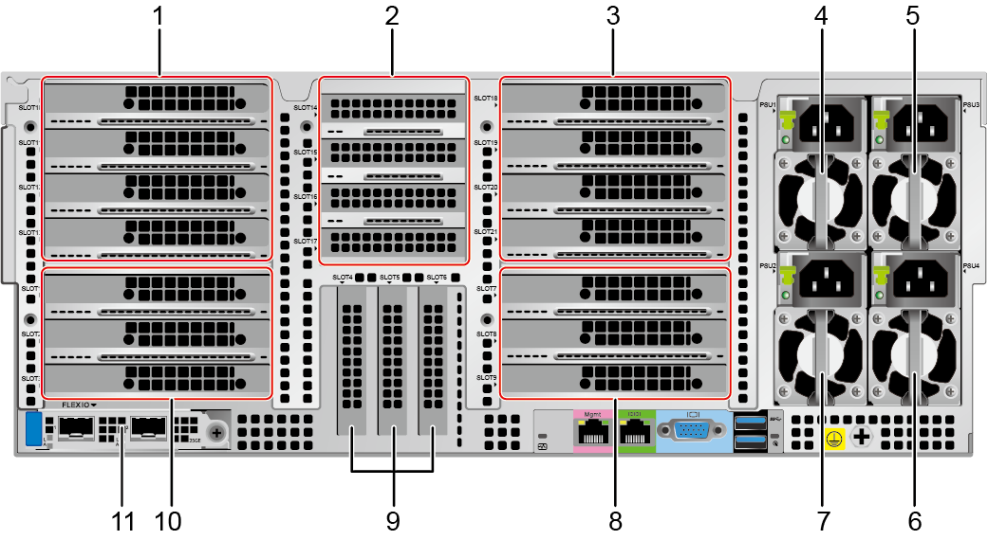
Figure 5-22 Rear view
