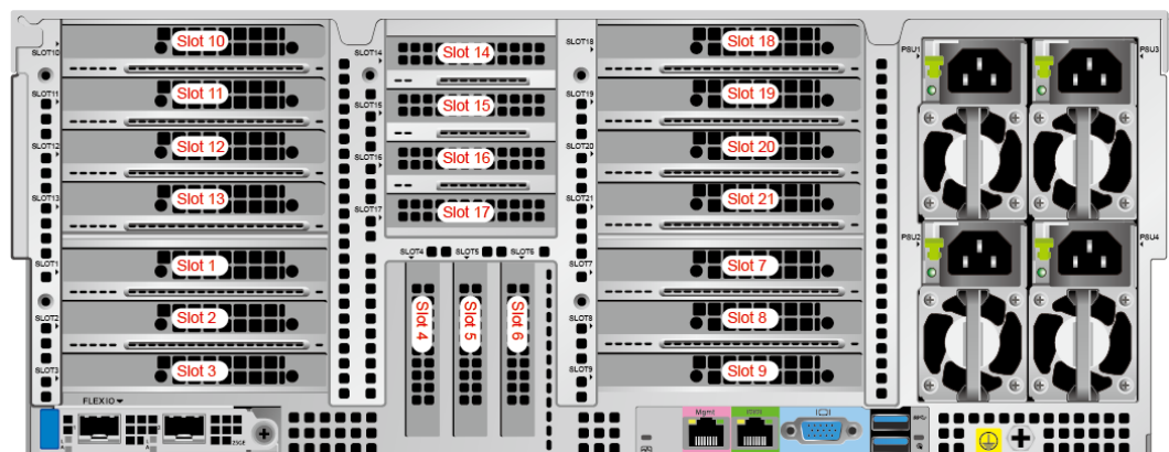
Figure 5-51 PCIe slots
