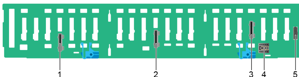
Figure 5-61 24 x 2.5" drive pass-through backplane
