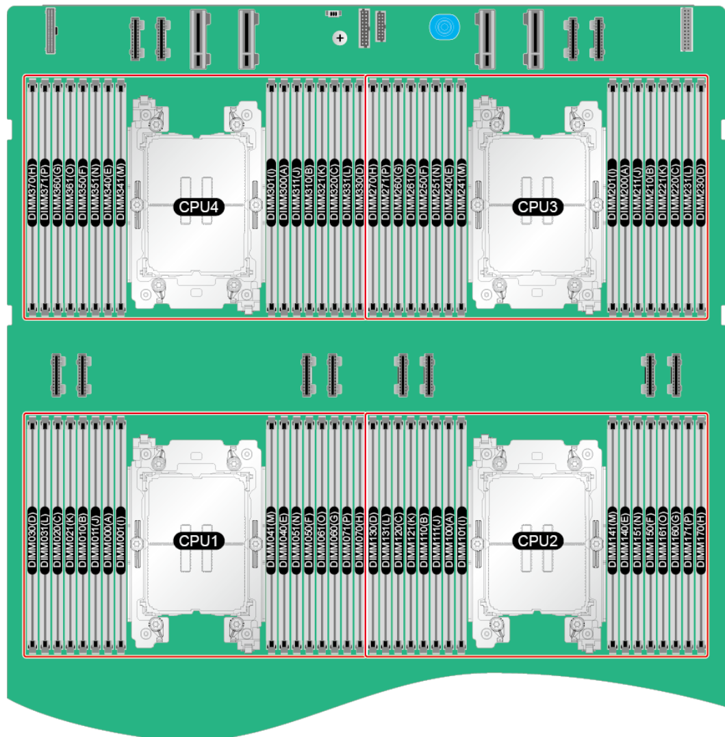
Figure 5-30 Positions of the memory modules
