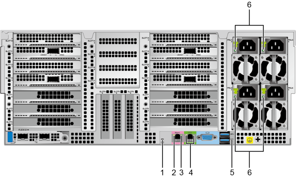
Figure 5-25 Indicators on the rear panel
