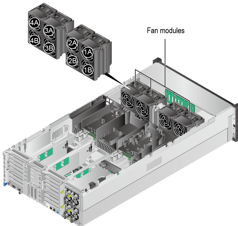
Figure 5-56 Positions of the fan modules
