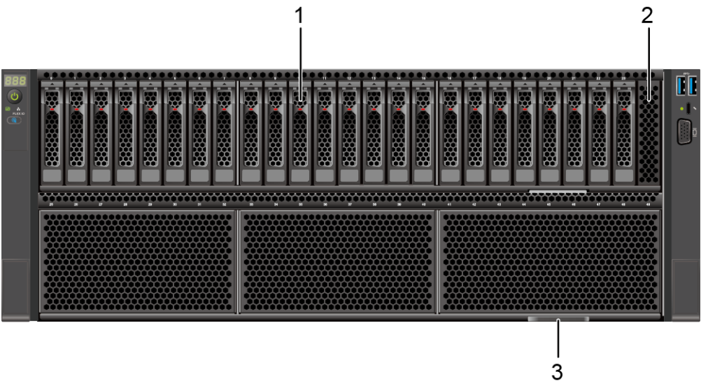
Figure 5-3 Front view
