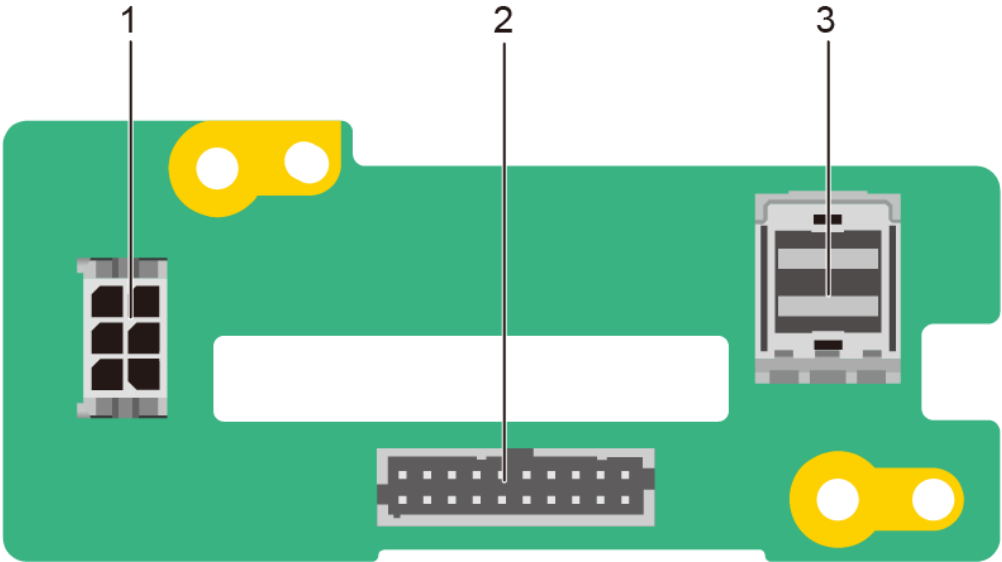
Figure 5-65 2 x 2.5" drive backplane
