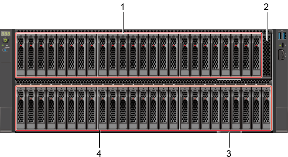
Figure 5-6 Front view
