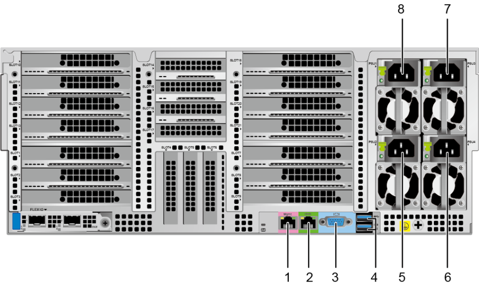
Figure 5-26 Ports on the rear panel
