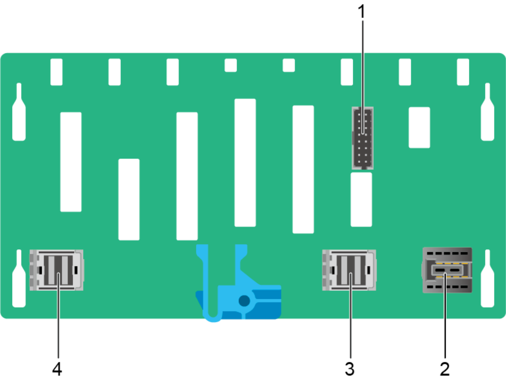
Figure 5-59 8 x 2.5" drive pass-through backplane
