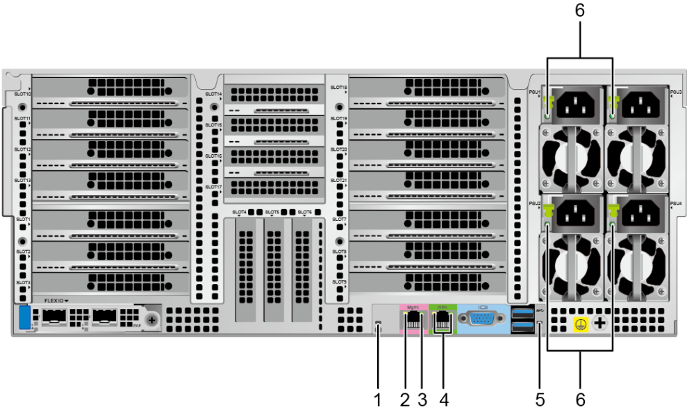
Figure 5-24 Indicators on the rear panel
