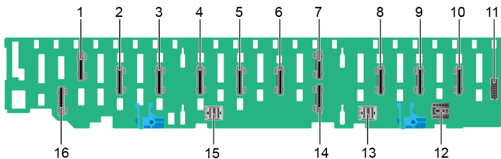
Figure 5-62 24 x 2.5" drive NVMe backplane
