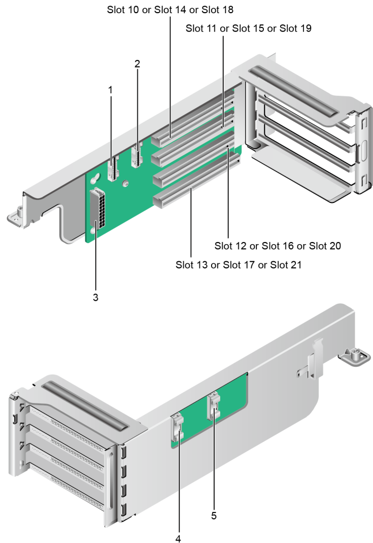
Figure 5-53 PCIe riser card 2
