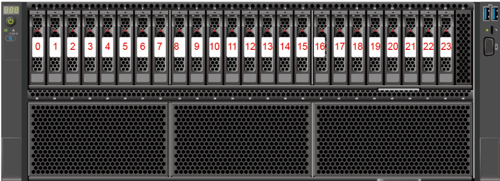
Figure 5-44 Drive numbering
