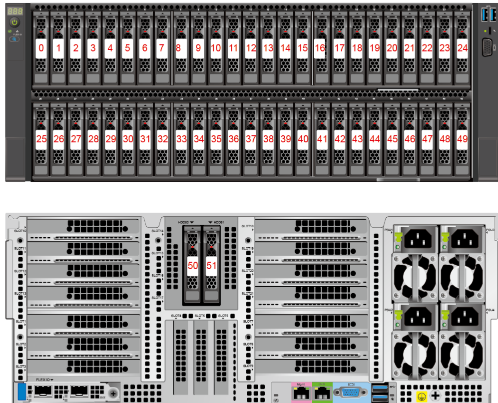
Figure 5-47 Drive numbering
