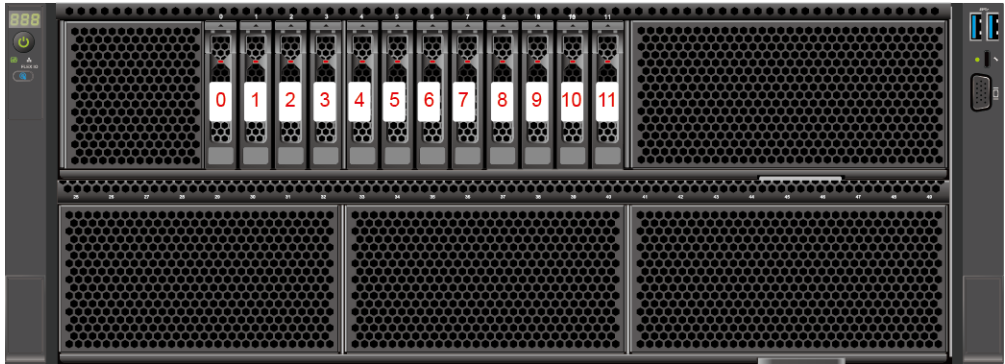
Figure 5-37 Drive numbering
