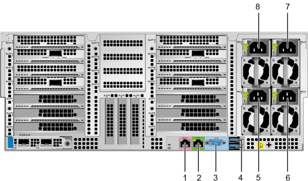
Figure 5-27 Ports on the rear panel
