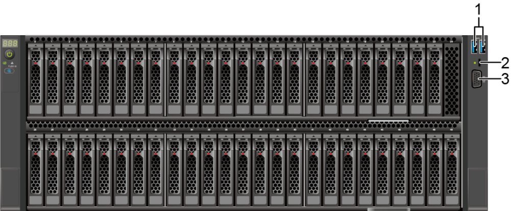
Figure 5-21 Ports on the front panel
