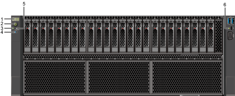
Figure 5-10 Indicators and buttons on the front panel
