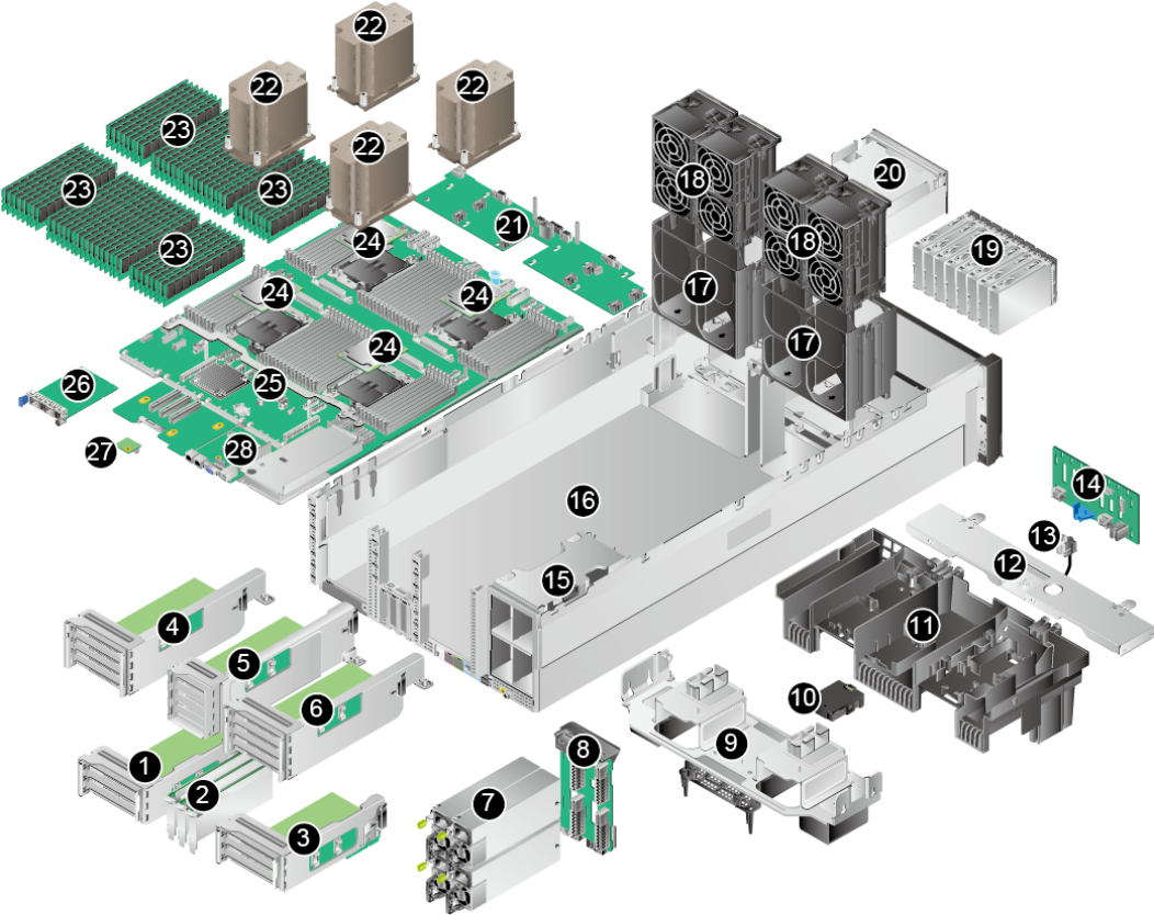
Figure 3-1 Physical structure of a server with 8 x 2.5" drives (example)
