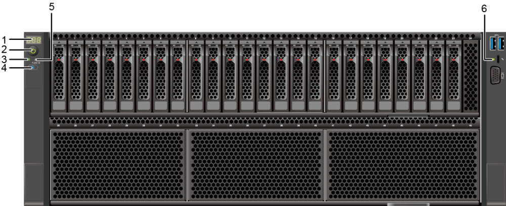
Figure 5-11 Indicators and buttons on the front panel
