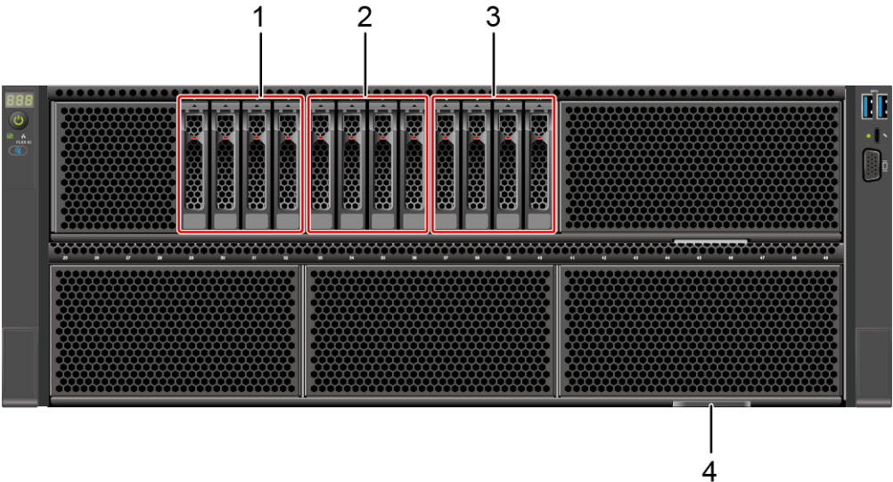
Figure 5-2 Front view
