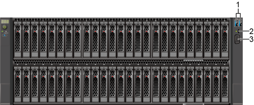
Figure 5-20 Ports on the front panel
