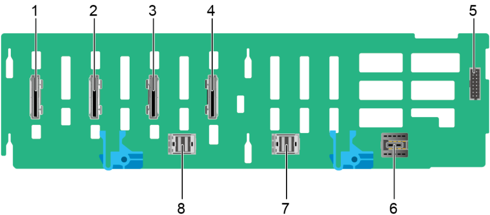
Figure 5-60 12 x 2.5" drive pass-through backplane
