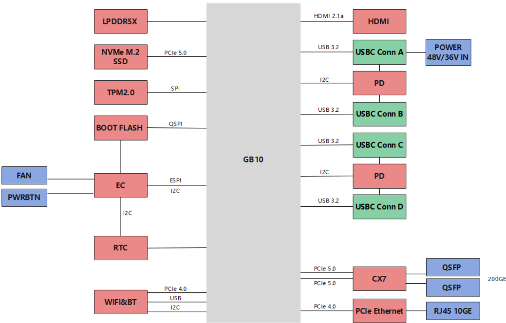
Figure 3-1 FusionXpark system block diagram
