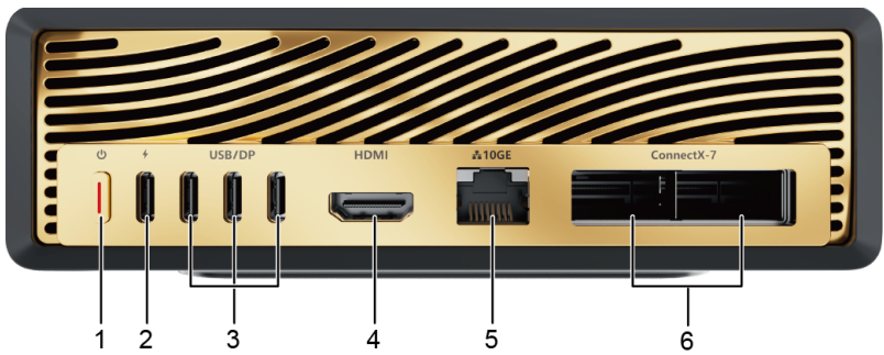
Figure 3-4 Buttons and ports
