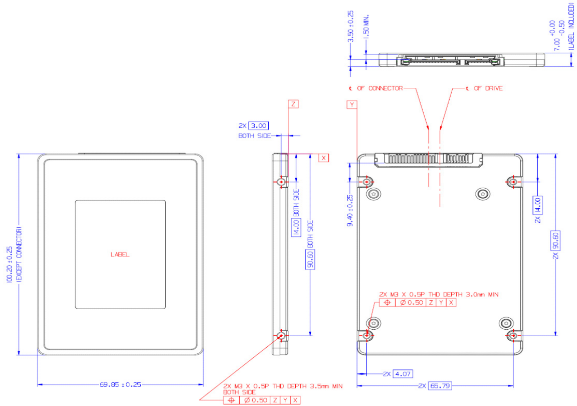
Figure 2. Physical Dimension
